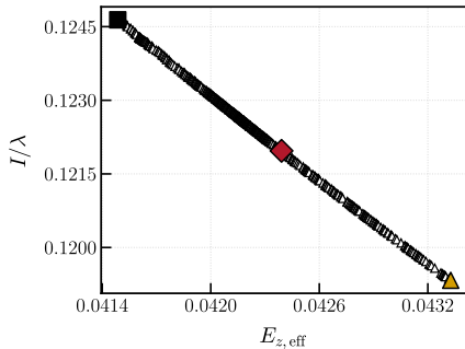
C028: E_{z,\text{eff}} vs. I/\lambda
