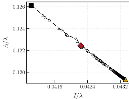
C029: I/\lambda vs. A/\lambda
