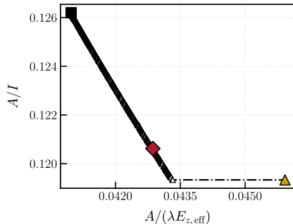
C030: A/(\lambda E_{z,\text{eff}}) vs. A/I
