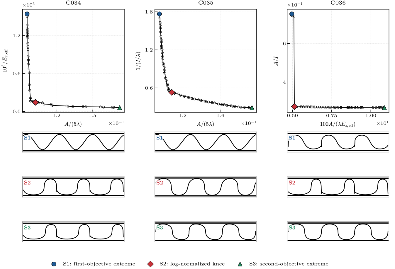
Figure B12: New coupled size--shape cases C034–C036. The ten variables comprise seven rational-shape coordinates, pitch, centreline height and common paper thickness; all candidates satisfy the 0.9 mm radius condition.
