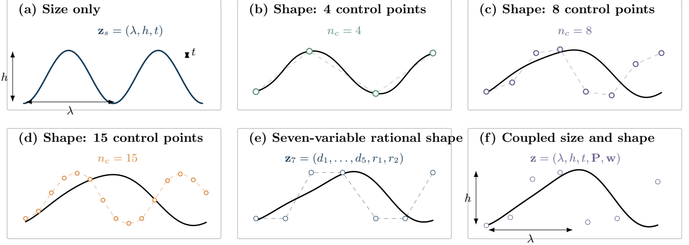
Figure 4: Optimization cases distinguished in the numerical archive. Size-only cases vary the physical envelope; shape-only cases vary 4, 8 or 15 control points at fixed envelope; the seven-variable rational construction varies five normalized spacings and two weights; and coupled cases vary size and shape together. Control polygons are schematic, while the objective fronts reported later are read directly from the archived CSV files.
