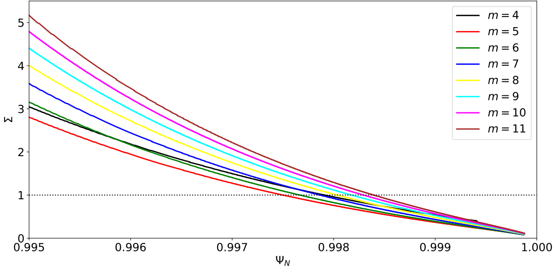
FIG. 12. The shielding factors, \Sigma , at the n = 1 rational surfaces, plotted as functions of the normalized poloidal magnetic fluxes, \Psi_N , at the surfaces, in the outer part of a model ITER pedestal.
