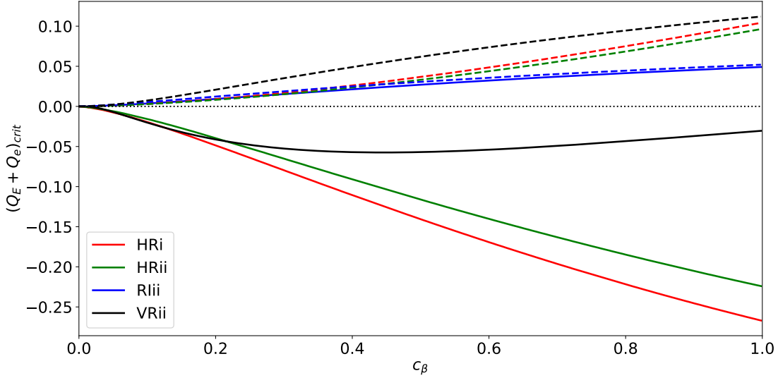
FIG. 6. The critical value of the normalized electron fluid rotation frequency at the rational surface, Q_E + Q_e , at which the real (solid curves) and imaginary ( imaginary dashed curves) parts of the layer response index pass through zero, plotted as a function of c_\beta for the four response regimes specified in Table I.
