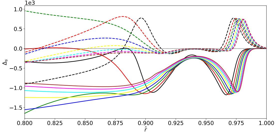
FIG. 10. The real (solid curves) and imaginary (dashed curves) parts of the layer response indices, \Delta_s , at the n = 1 rational surfaces, plotted as functions of the normalized minor radii, \hat{r} , of the surfaces, in a model ITER pedestal. Different colored curves correspond to different poloidal mode numbers according to the legend in Fig. 12.
