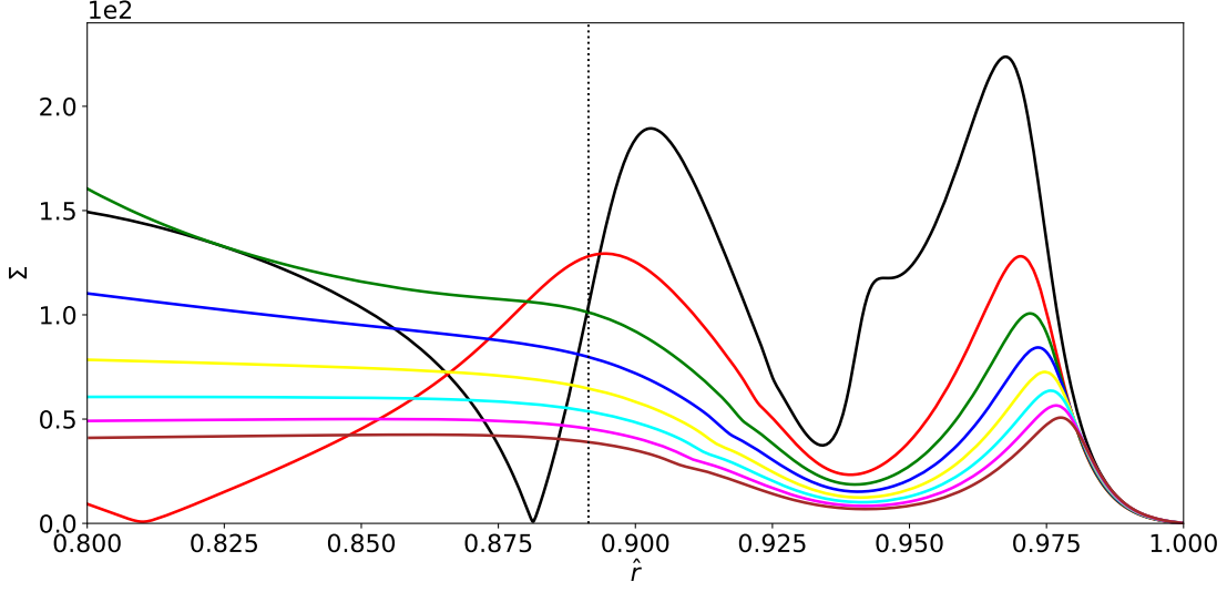
FIG. 11. The shielding factors, \Sigma , at the n = 1 rational surfaces, plotted as functions of the normalized minor radii, \hat{r} , of the surfaces, in a model ITER pedestal. Different colored curves correspond to different poloidal mode numbers according to the legend in Fig. 12. The vertical dotted line indicates the radius at which \omega_{\perp e} \equiv \omega_E + \omega_{*e} = 0 .
