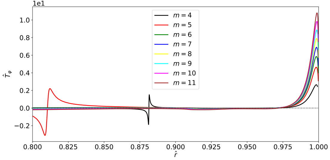
FIG. 13. The normalized toroidal electromagnetic torques, \hat{T}_\phi , at the n = 1 rational surfaces, plotted as functions of the normalized minor radii, \hat{r} , of the surfaces, in a model ITER pedestal.
