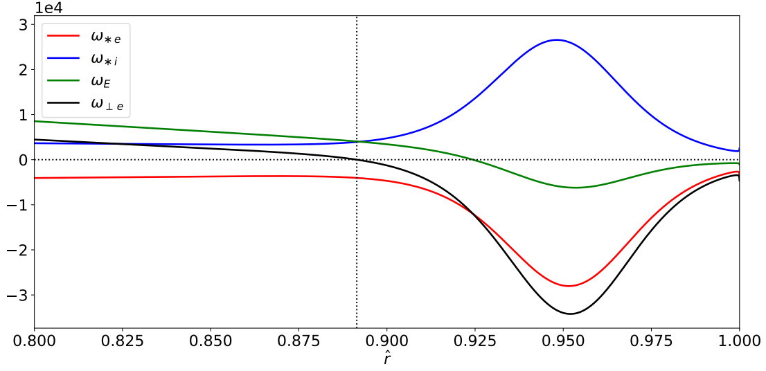
FIG. 8. Rotation frequency profiles in a model ITER pedestal. Here, \omega_{*e} is the electron diamagnetic frequency, \omega_{*i} the ion diamagnetic frequency, \omega_E the \mathbf{E} \times \mathbf{B} frequency, and \omega_{\perp e} \equiv \omega_E + \omega_{*e} the electron fluid rotation frequency. The vertical dotted line indicates the radius at which \omega_{\perp e} = 0 . All frequencies are measured in units of radians per second.
