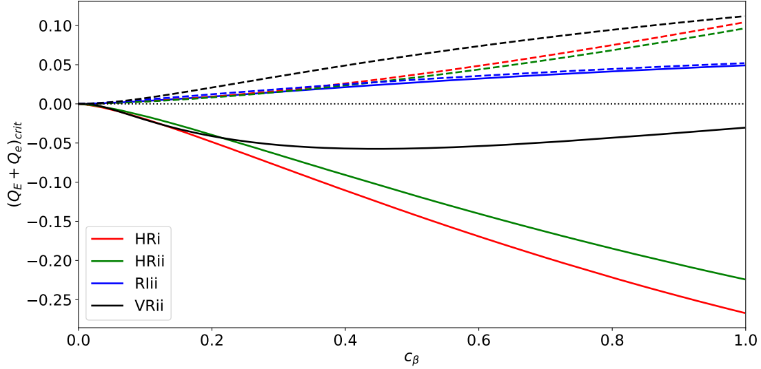
FIG. 6. The critical value of the normalized electron fluid rotation frequency at the rational surface, Q_E + Q_e , at which the real (solid curves) and imaginary (imaginary curves) parts of the layer response index pass through zero, plotted as a function of c_\beta for the four response regimes specified in Table ??.
