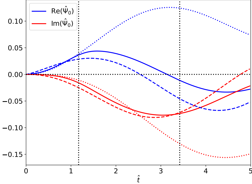
FIG. 9. Driven reconnected magnetic flux at relatively early times in Reconnection Scenario 1. Here, the solid curves show the fully numerical solution, the dotted curves show the analytic solution in the inertial response regime, and the dashed curves show the analytic solution in the viscous-inertial response regime. The two dotted vertical lines show the approximate times at which the transitions from the inertial to the viscous-inertial, and from the viscous-inertial to the viscous-resistive, response regimes occur, in order from the left to the right.
