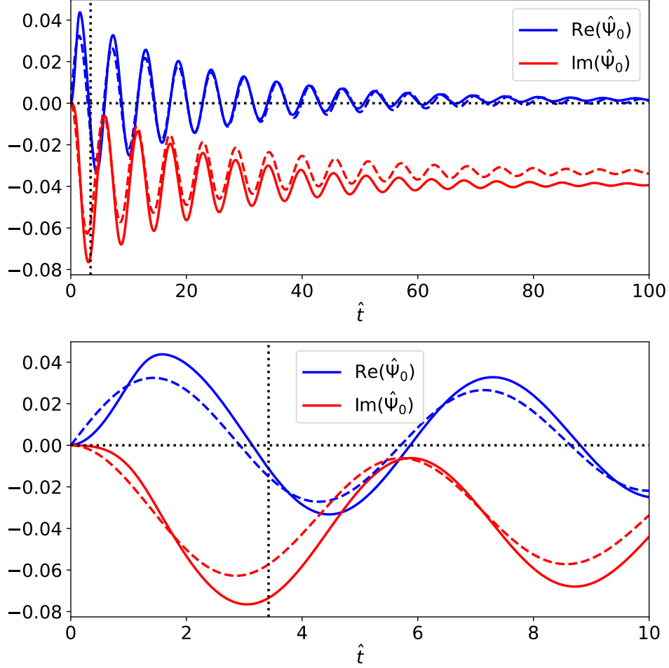
FIG. 10. Driven reconnected magnetic flux at relatively late times in Reconnection Scenario 1. Here, the solid curves show the numerical solution, whereas the dashed curves show the analytic solution in the viscous-resistive response regime. The vertical dotted line shows the approximate time at which the transition from the viscous-inertial to the viscous-resistive response regime occurs.
