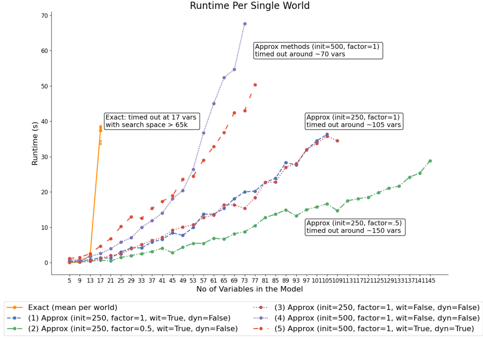
Figure 10: Per-world runtime against problem size. The exact method (orange) times out at 17 variables; approximate methods continue, with reach controlled by total sample budget. Five approximate configurations vary initial sample size, the linear-growth factor \alpha , the witness ablation, and dynamic cardinality bounds; see Benchmark protocol.
