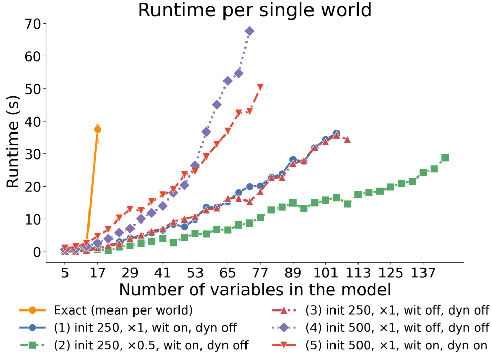
Figure 6: Per-world runtime against problem size. The exact method (orange) times out at 17 variables; approximate methods continue, with reach controlled by total sample budget. Five approximate configurations vary initial sample size, the linear-growth factor \alpha , the witness ablation, and dynamic cardinality bounds; see Benchmark protocol.
