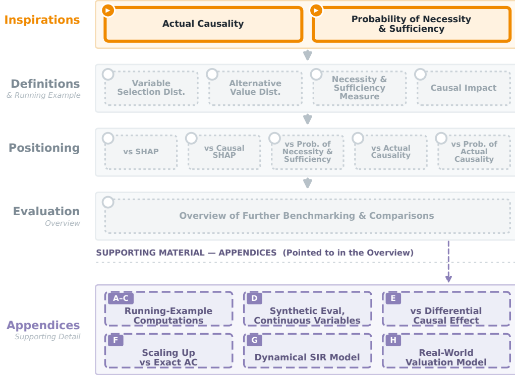
Figure 1: Roadmap of the paper. An overview of the argument, here at its starting point. PCI builds on two ideas — actual causality and the probability of necessity and sufficiency (top tier, highlighted as the current stage). From there the paper develops the motivations (Section 2), defines PCI (Section 3), positions it against SHAP, Causal SHAP, PNS, actual causality, and the probability of actual causation (Sections 4 to 6), and closes with an empirical overview (Section 7); the running-example computations and benchmark protocols are deferred to the appendices, to which that overview points.
