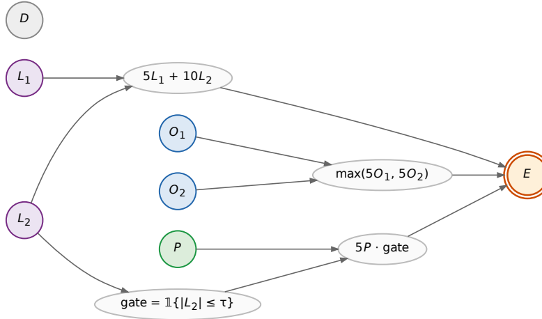
Figure 1: Design C. Roots (circles) are independent draws: L_1, L_2 \sim \mathcal{N}(0, 1) (linear, purple); O_1, O_2 \sim \mathcal{N}(1, 1) (overdetermined via max, blue); P \sim \mathcal{N}(0, 1) (gated by |L_2| \leq \tau , green); D \sim \mathcal{N}(0, 1) (irrelevance control, grey). Mediators (white ellipses) carry the deterministic functions of their parents. Outcome E (orange double-circle) is the sum \text{lin} + \text{od} + \text{p\_branch} . The variable D has no outgoing edges by construction.
