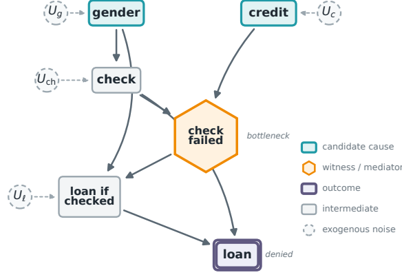
Figure 3: Causal structure of the OBCB loan model (Example 6). Node shape and colour encode role: the candidate causes gender and credit (teal boxes), the witness check-failed (gold hexagon), and the outcome loan (purple double box); intermediate variables are grey. Dashed circles are the exogenous noise U_V feeding each stochastic mechanism; the deterministic nodes check-failed and loan carry none. Note that check reaches loan along two routes: through the check-failed bottleneck and directly as the screening gate ( loan = loan\text{-}if\text{-}checked \cdot check ). PCI holds the bottleneck witness fixed to keep these two routes distinct.
