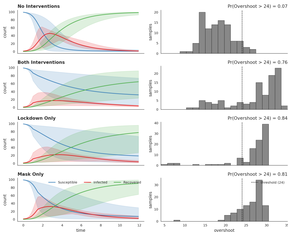
Figure 20: SIR trajectories and overshoot distributions under the four interventional regimes (no interventions, both policies, lockdown only, mask only). Left: posterior bands for susceptible (blue), infectious (red) and recovered (green) over time, with the lockdown enacted at t = 1 and the mask mandate at t = 1.5 . Right: per-regime histograms of the overshoot, with the 24-overshoot threshold marked. Either policy on its own leaves the infectious peak essentially intact; only the joint regime suppresses it appreciably, yet the lockdown-only and mask-only overshoot probabilities are near-indistinguishable: the asymmetric joint efficiency that PCI disentangles.
