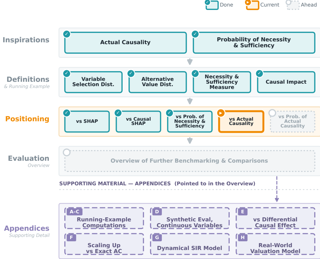
Figure 7: Roadmap: relating to actual causality (current stage). The next section establishes the formal correspondence between the PCI kernel and Halpern’s actual cause. It then positions PCI against Pearl’s probability of actual causation (Section 6), before the empirical evaluation.
