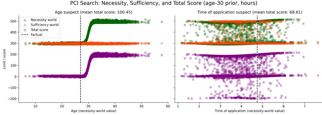
Figure 17: PCI search for the canonical setting (age-30 prior, hours), with age (left) and time of application (right) as the active suspect. Necessity-world (green) and sufficiency-world (orange) limit samples and the total score (purple) are plotted against the necessity-world value of the suspect; the dashed line marks the factual. The necessity world departs from factual along the deterministic response while the sufficiency world stays near it; each panel title gives the mean total score.
