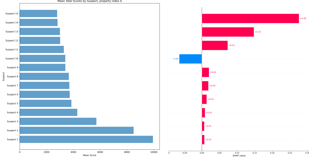
Figure 14: PCI vs. SHAP on a deployed automated valuation model. Left: PCI’s context-sensitive attribution across the AVM’s internal variables. Right: SHAP concentrates responsibility on a few downstream variables. Full pipeline and anonymized structure in Appendix H.
