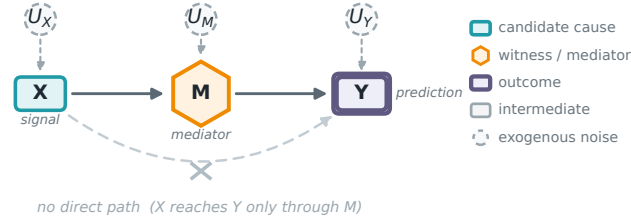
Figure 6: The signal-with-mediation model. X (teal) reaches the outcome Y (purple double box) only through the mediator M (gold hexagon); the faded, crossed-out arc marks the absent direct path X \rightarrow Y . Dashed circles are the independent Gaussian noises U_X, U_M, U_Y of Eqs. (5) to (7). That one missing edge is what desideratum D-MXY asks an attribution to register: M acts on Y directly, whereas X acts only at one remove.
