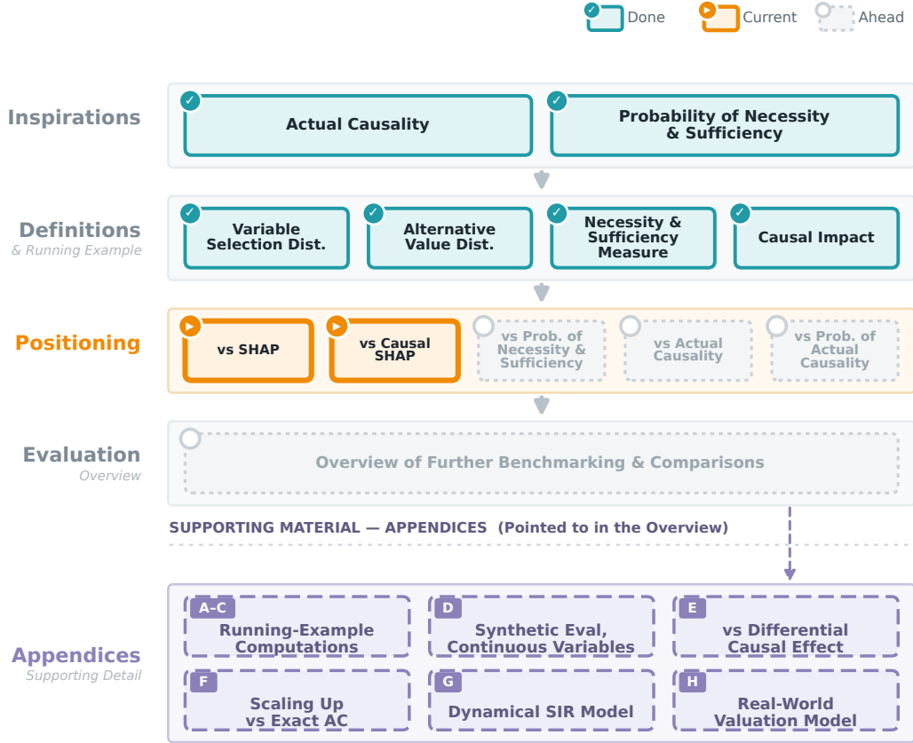
Figure 5: Roadmap: positioning against SHAP (current stage). With PCI defined, the next section compares it with SHAP, Causal SHAP, ATE, and CATE on two worked examples. The argument then establishes the formal relation to actual causality (Section 5) and to Pearl’s probability of actual causation, before the empirical evaluation.
