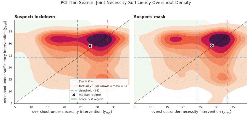
Figure 13: PCI separates interacting policies on a continuous dynamical outcome. Joint necessity-sufficiency over the two policies for the peak-overshoot event; lockdown carries roughly twice the responsibility of masking where but-for analysis ties them. Full model and query in Appendix G.
