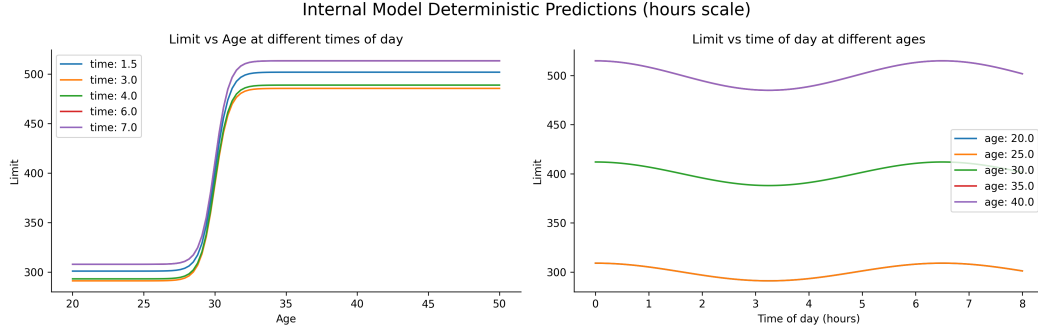
Figure 16: Deterministic component of the credit-limit model (Example 37), on the hours scale: limit vs. age at several times of day (left) and limit vs. time of day at several ages (right). Age dominates the limit, with a small sinusoidal modulation from time of day; the minute scale is identical modulo a linear reparameterisation (verified in the notebook).
