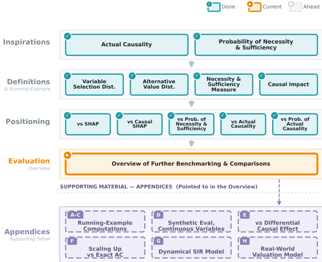
Figure 10: Roadmap: empirical evaluation (current stage). The next, final phase evaluates PCI across four settings, reading each result at a glance with the full protocols and derivations in the appendices (dashed band). Section 8 then closes the paper.
