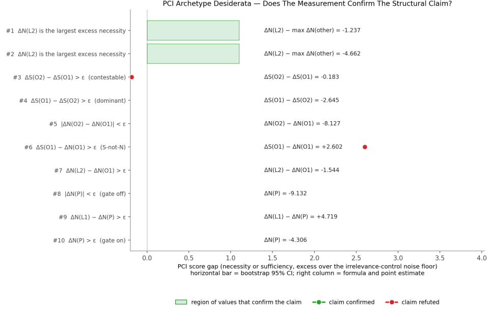
Figure 11: PCI recovers the actual-causality verdicts on a four-archetype synthetic model. Each row is one archetype desideratum (linear necessity/sufficiency, overdetermination, preemption, irrelevance control); the dot is the bootstrap point estimate of the relevant \Delta score, the bar its 95% CI, and the green band the pass region given the data-derived threshold \epsilon \approx 0.151 . All ten dots fall inside their bands. Full model, estimator, and per-row analysis in Appendix D.
