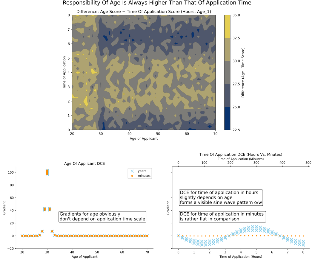
Figure 18: PCI vs. DCE on the credit-limit grid (age-30 prior, hours). Top : difference between the PCI scores for age and for time of application; positive everywhere, largest near the steep region of the age-limit sigmoid and for ages far from the prior mean, so age is always the more responsible variable. Bottom : DCE for age (left) and time of application (right) on both unit scales. Age has the larger absolute DCE only inside the narrow steep region of the sigmoid; elsewhere time of application dominates on the hour scale and goes comparatively flat on the minute scale, illustrating DCE’s shape and unit sensitivity.
