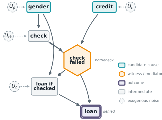
Figure 2: Causal structure of the OBCB loan model (Example 6). Node shape and colour encode role: the candidate causes gender and credit (teal boxes), the witness check-failed (gold hexagon), and the outcome loan (purple double box); intermediate variables are grey. Dashed circles are the exogenous noise U_V feeding each stochastic mechanism —the deterministic nodes check-failed and loan carry none. Note that check reaches loan along two routes: through the check-failed bottleneck and directly as the screening gate ( loan = loan-if-checked \cdot check ). PCI holds the bottleneck witness fixed to keep these two routes distinct.
