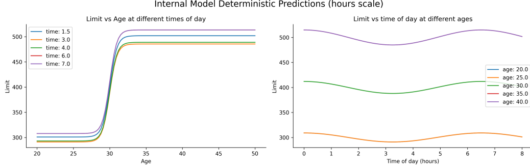
Figure 16: Deterministic component of the credit-limit model (Example 36), on the hours scale: limit vs. age at several times of day (left) and limit vs. time of day at several ages (right). Age dominates the limit, with a small sinusoidal modulation from time of day; the minute scale is identical modulo a linear reparameterisation (verified in the notebook).
