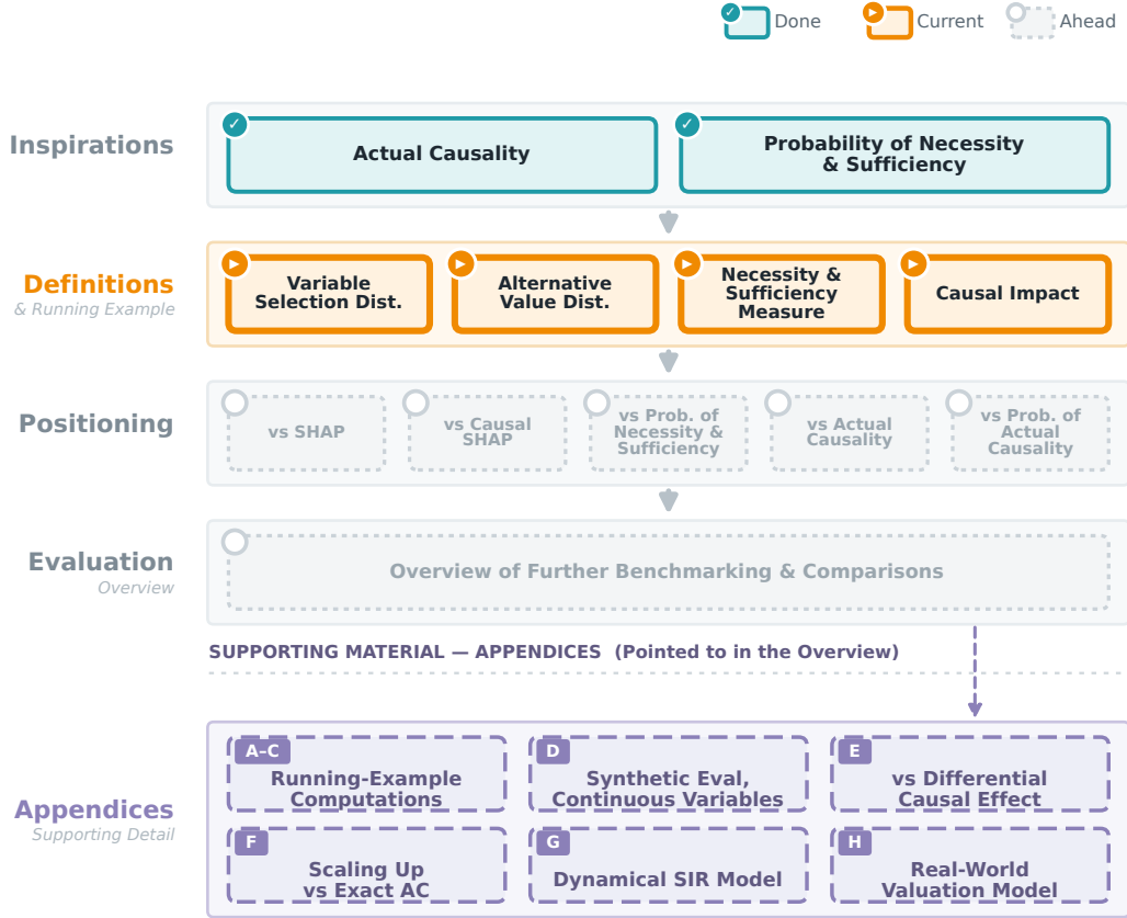
Figure 3: Roadmap: defining PCI (current stage). With the motivations in place, the next section introduces the framework — the variable selection distribution \Gamma , the alternative-value distribution \Delta , and the causal impact function ci . It then positions PCI against the SHAP family (Section 4), against actual causality and its probabilistic wrappers, and closes with the empirical evaluation.
