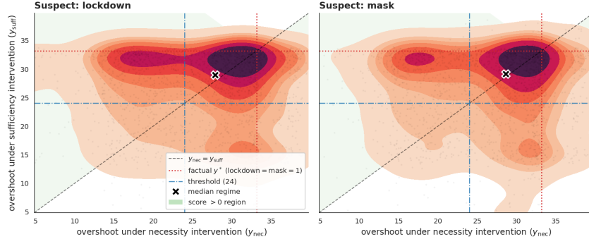
Figure 13: PCI separates interacting policies on a continuous dynamical outcome. Joint necessity-sufficiency over the two policies for the peak-overshoot event; lockdown carries roughly twice the responsibility of masking where but-for analysis ties them. Full model and query in Appendix G.
