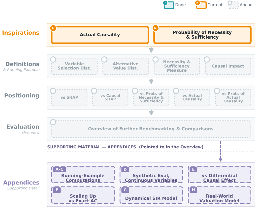
Figure 1: Roadmap of the paper. An overview of the argument, here at its starting point. PCI builds on two ideas — actual causality and the probability of necessity and sufficiency (top tier, highlighted as the current stage). From there the paper develops the motivations (Section 2), defines PCI (Section 3), positions it against SHAP, Causal SHAP, PNS, actual causality, and the probability of actual causation (Sections 4 to 6), and closes with an empirical overview (Section 7); the running-example computations and benchmark protocols are deferred to the appendices, to which that overview points.
