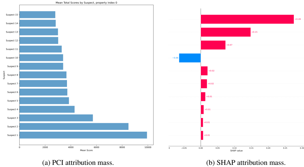
Figure 17: Attribution distributions on the AVN, with feature labels anonymised. Left: PCI attribution mass spread across upstream causal variables (suspects 1–15, ranked by mean total score). Right: SHAP attribution mass concentrated on a small number of downstream variables. The qualitative pattern matches the controlled-setting comparison of Section 5.
