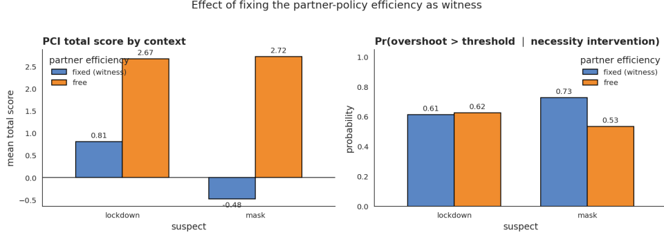
Figure 15: Different-contexts experiment. Bars compare PCI total score (left) and \Pr(\text{overshoot} > 24 \mid \text{necessity}) (right) when the partner-policy efficiency variable is fixed as a witness versus left free. Lockdown’s score is positive in both regimes; mask’s score flips sign across regimes, indicating that mask is a context-sensitive rather than a robust cause.
