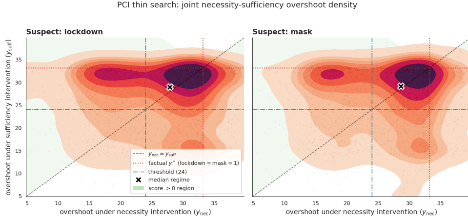
Figure 14: Joint necessity-sufficiency overshoot density per suspect. Each point is one sampled regime. Dotted red cross-hair: factual y^* at lockdown = mask = 1 (the high-overshoot anchor); dash-dot blue: the 24-overshoot threshold; dashed black: y_{\text{nec}} = y_{\text{suff}} . A regime contributes positively to the PCI total iff it sits further from the red cross-hair along the necessity axis than along the sufficiency axis. The lockdown density is shifted toward smaller y_{\text{nec}} relative to y_{\text{suff}} (the cause signature on this geometry); the mask density sits closer to the diagonal.
