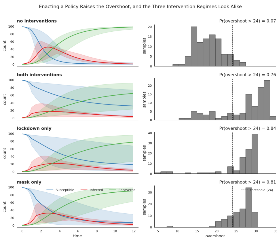
Figure 18: SIR trajectories and overshoot distributions under the four interventional regimes (no interventions, both policies, lockdown only, mask only). Left: posterior bands for susceptible (blue), infectious (red) and recovered (green) over time, with the lockdown enacted at t = 1 and the mask mandate at t = 1.5 . Right: per-regime histograms of the overshoot, with the 24-overshoot threshold marked. Either policy on its own leaves the infectious peak essentially intact; only the joint regime suppresses it appreciably, yet the lockdown-only and mask-only overshoot probabilities are near-indistinguishable: the asymmetric joint efficiency that PCI disentangles.
