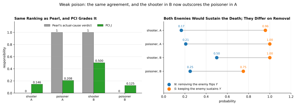
Figure 13: Weak-poison variant, laid out as Figure 12. Pearl scores both operative enemies at 1 and cannot separate the scenarios; PCI separates them, ranking the shooter in Scenario B ( 1/2 ) above the poisoner in Scenario A ( 5/24 ).
