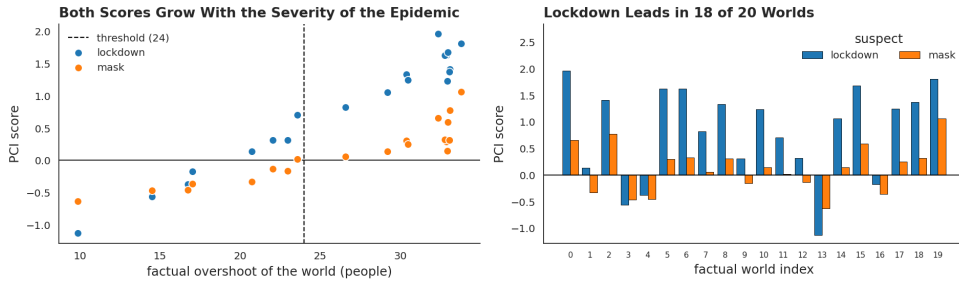
Figure 20: The single-world verdict across 20 factual worlds drawn from the prior. Left: PCI score against the world's factual overshoot, for each suspect. Right: the per-world scores in draw order. Lockdown leads in 18 of the 20 worlds, with a mean gap of +0.701 (standard error 0.111).
