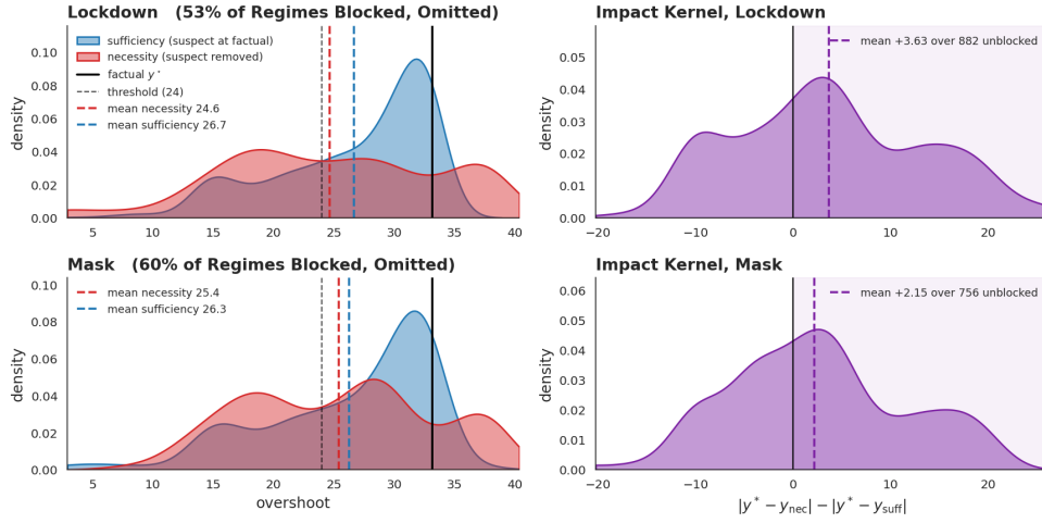
Figure 19: Impact-kernel densities per suspect. Left: the necessity world (suspect removed) spreads the overshoot away from y^* , while the sufficiency world (suspect held at factual) keeps it near y^* ; the printed means are the two columns of the table above. Right: the resulting per-draw impact kernel |y^* - y_{nec}| - |y^* - y_{suff}| , whose q^2 -scaled mean is the PCI score. The quarter of draws whose candidate set omits the suspect contribute zero and are excluded from the density.
