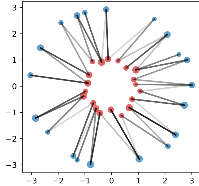
Plan optimal exact
