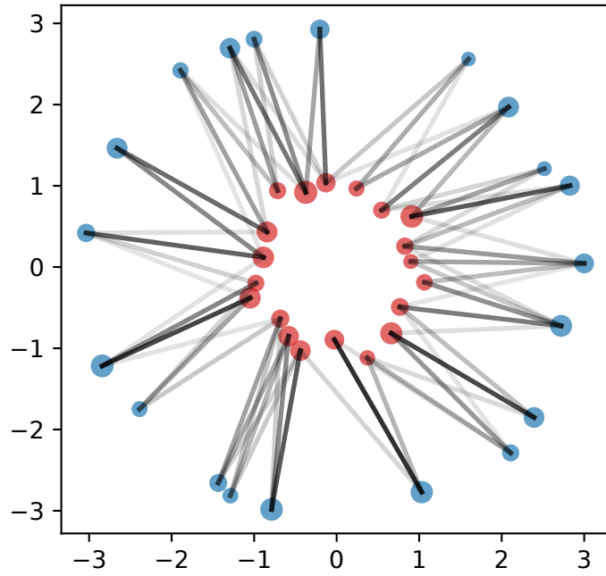
Plan optimal entropique \varepsilon = 0.2
