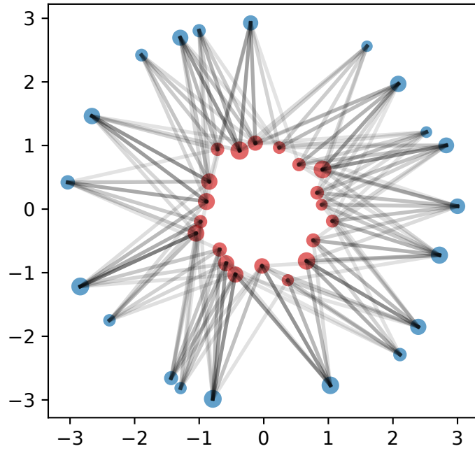
Plan optimal entropique \varepsilon = 1
