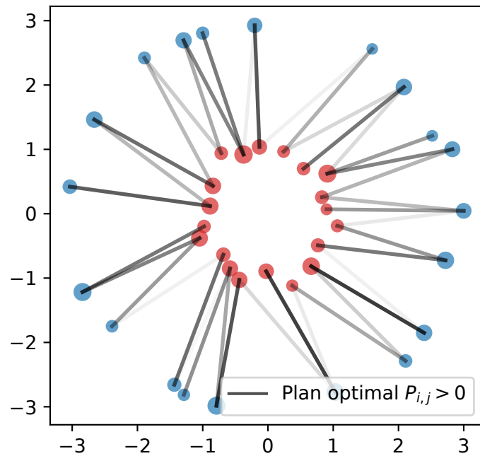
Plan optimal P
