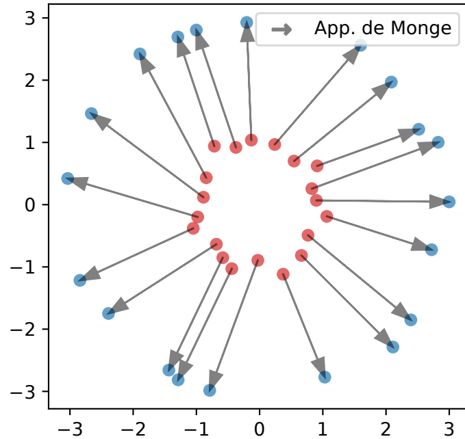
Application de Monge T
