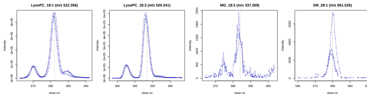
Figure 2: Extracted-ion chromatograms of the annotated biomarkers across the subset ( plotChromatogramsOverlay() ). Dashed line: annotated retention time.
