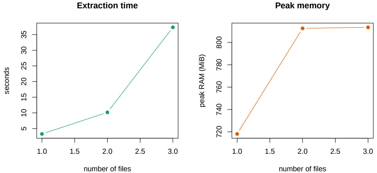
Figure 3: Targeted extraction time and peak RAM vs number of files.
