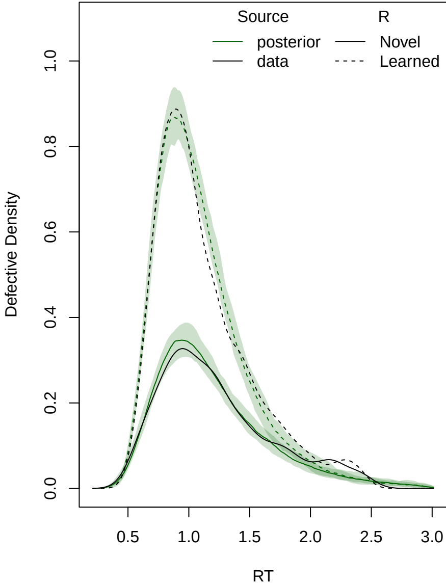
S=Learned
