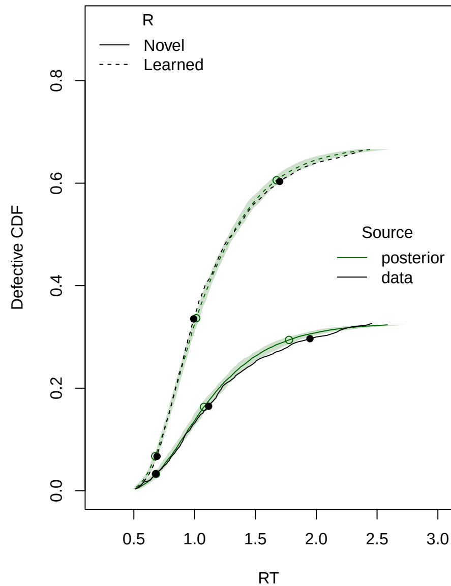
S=Learned
