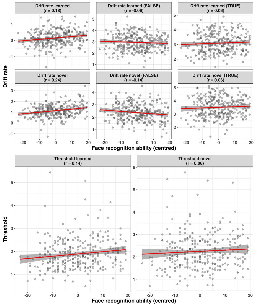
Figure 6. Correlations between face recognition ability and LBA parameters
