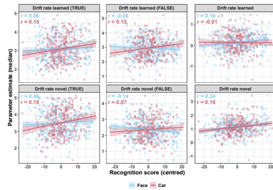
Figure 2. Median drift rate correlations with recognition ability
