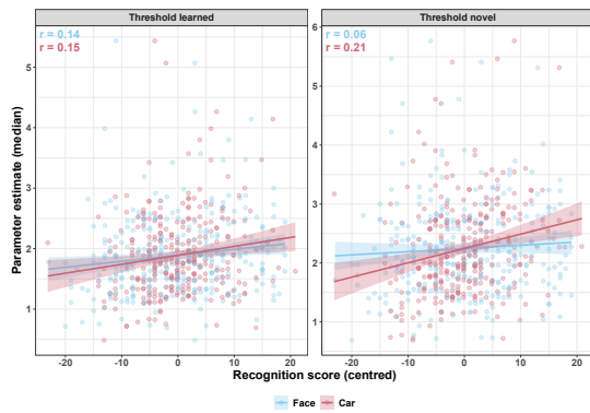
Figure 1. Median threshold correlations with recognition ability
