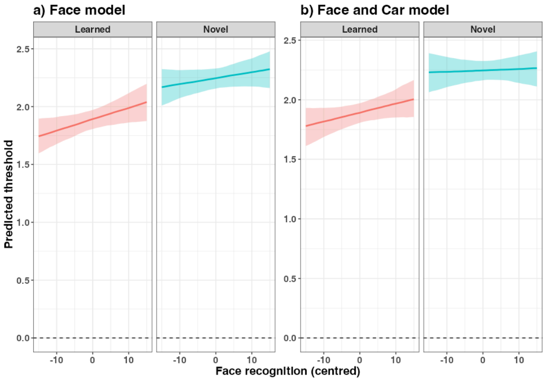
Figure 8. Predicted threshold values from face recognition ability scores for a) Face model and b) Face and Car model
