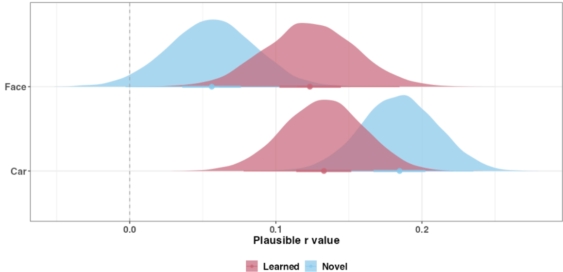
Figure 6. Plausible correlation values distributions between threshold by response and recognition abilities. Points denote the median of the distribution and error bars represent 95% quantile intervals.
