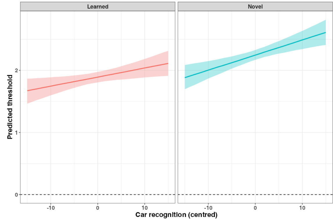
Figure 9. Predicted threshold values from car recognition ability scores for learned and novel responses
