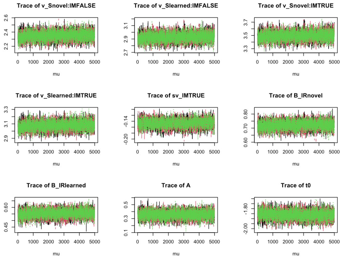
Figure 1. MCMC chains
