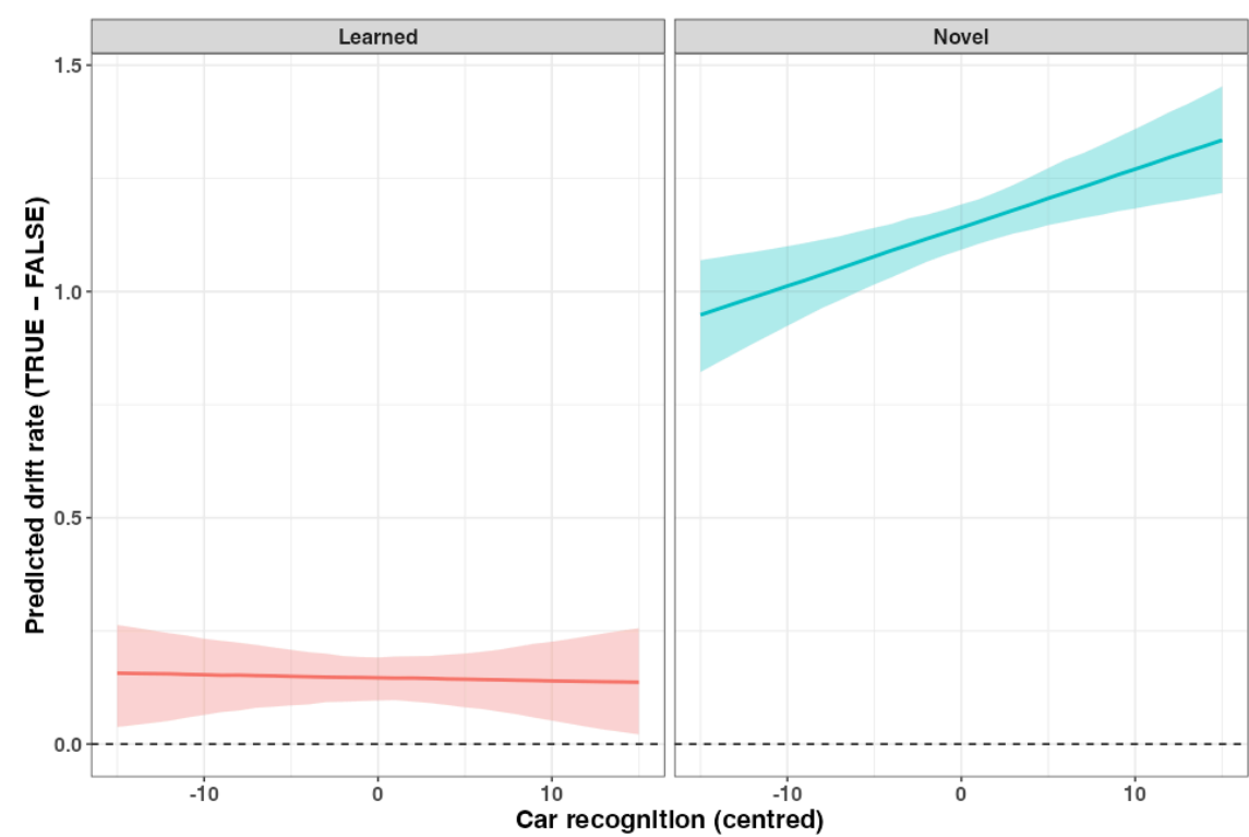
Figure 11. Predicted drift rate (TRUE-FALSE) values from car recognition ability for learned and novel faces
