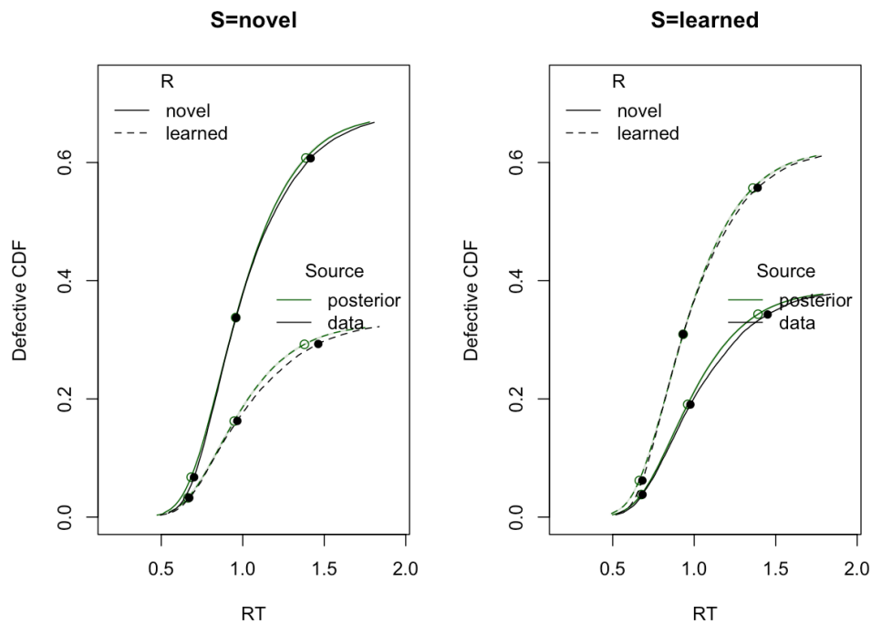
(a) CDF
