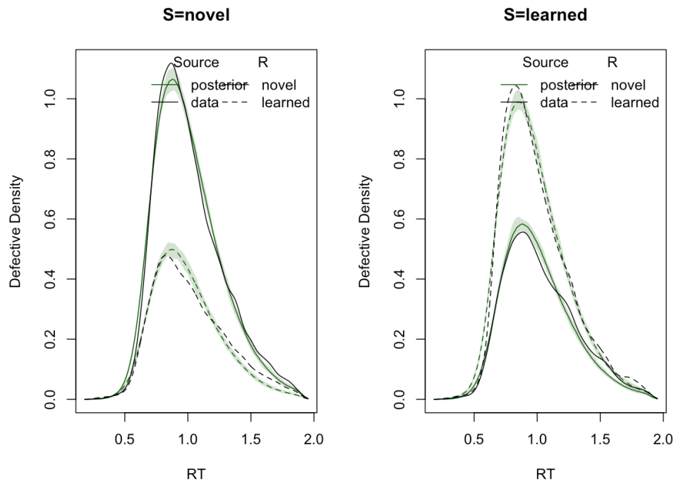
(b) Density
