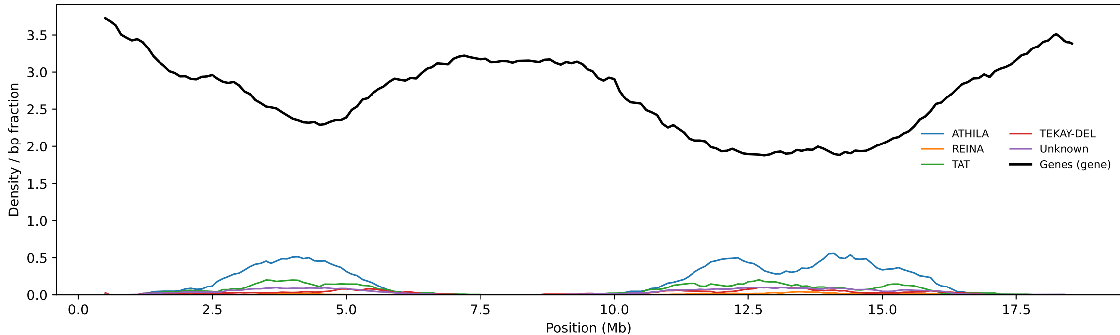
CP002687.1 - TE density
