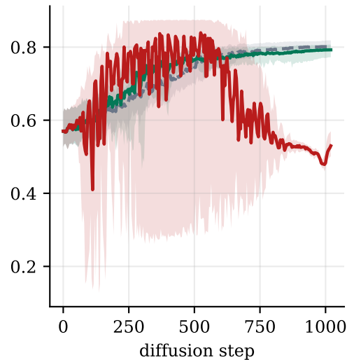
saturation p < 0.01
