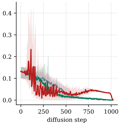
bit entropy
