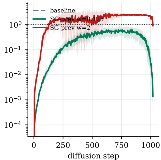
guidance / drift
