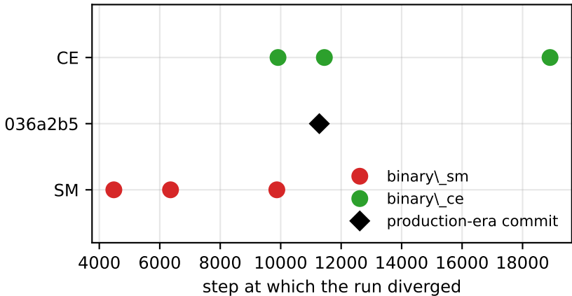
Time-to-divergence (3 seeds/arm)
