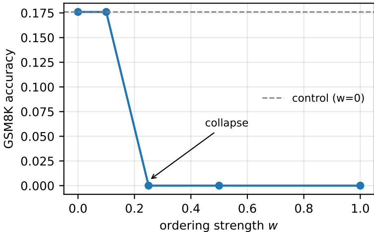
Ordering dose-response (l2r, n=250)
