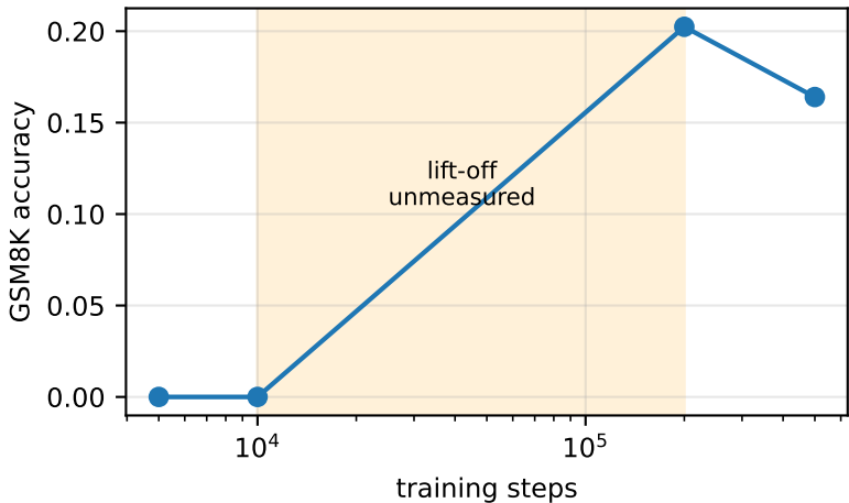
Accuracy vs training budget
