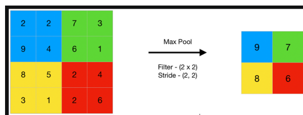
Figure 16.2: Max pooling
