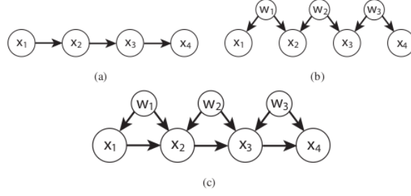
Figure 8.3: (a)→ AR(1) (b)→ MA(1) and (c)→ ARMA(1,1)
