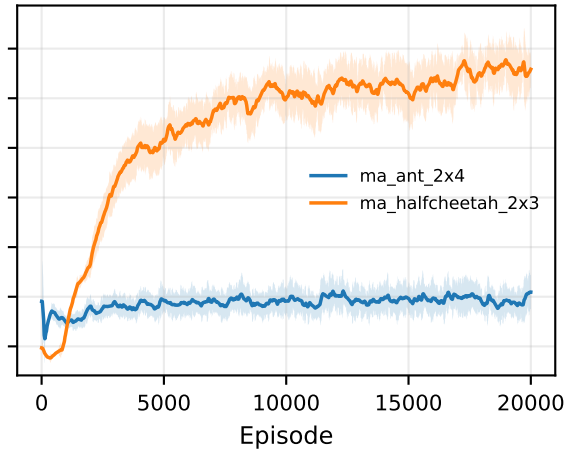
MADDPG
