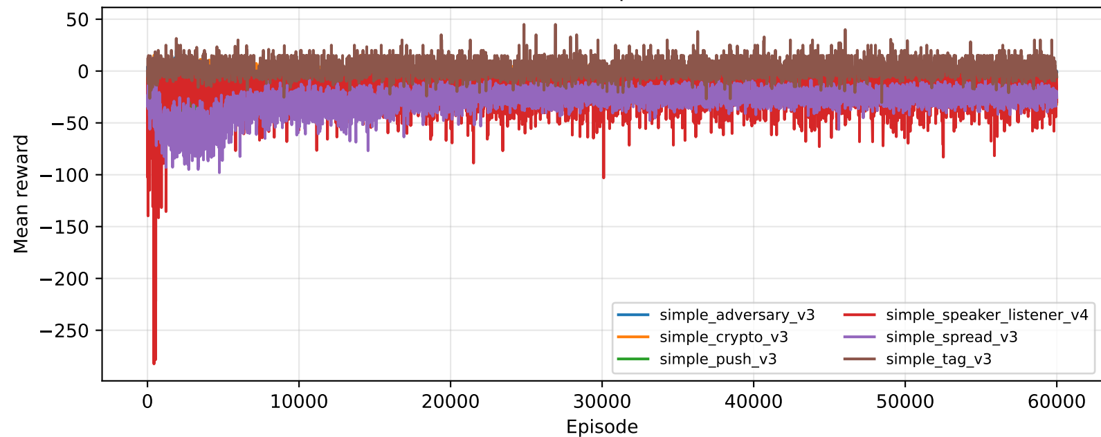
MADDPG mean episode reward
