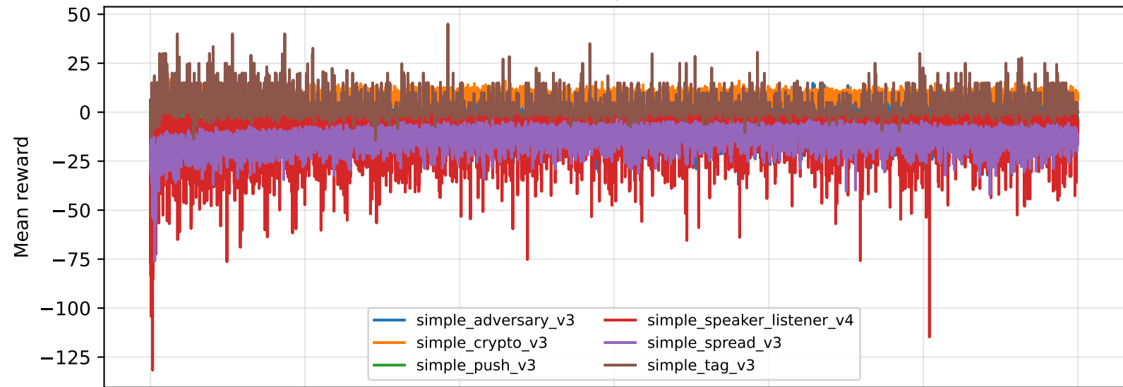
MAAC mean episode reward
