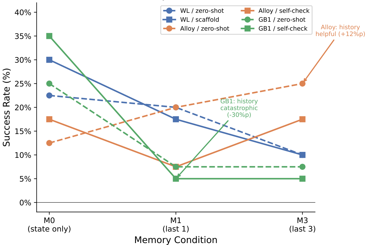
Effect of Edit History Access on Performance
