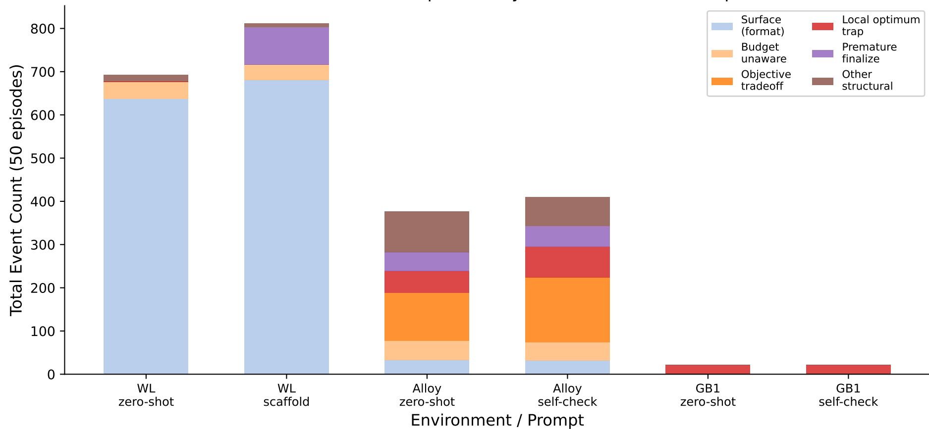
Failure Mode Decomposition by Environment and Prompt
