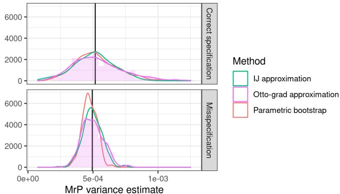
Figure 5: MrP Posterior Variance
