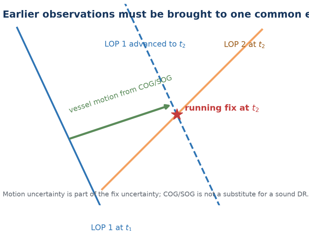
Figure 8. A numerical running fix advances the observation, not the celestial body, to a common vessel epoch.
