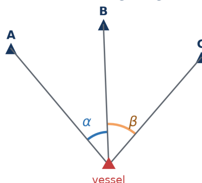
Two horizontal angles give a fix
