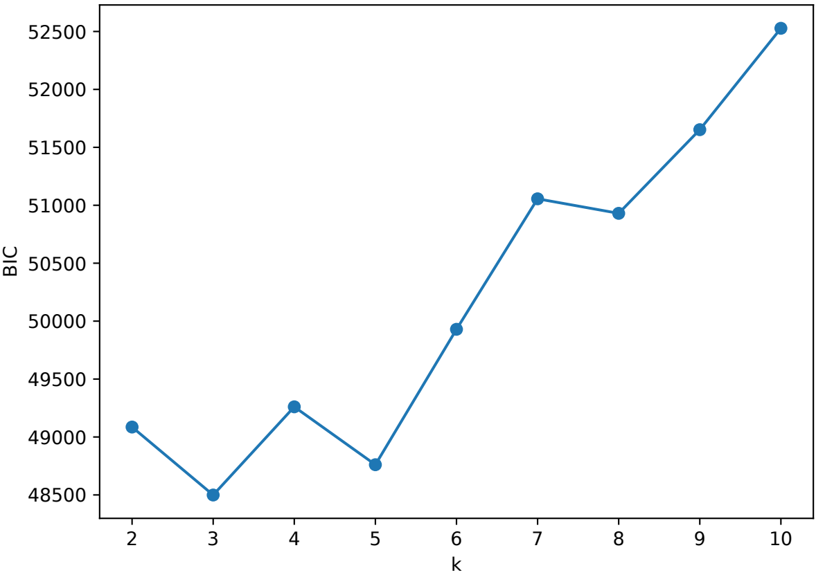
GMM: BIC vs k (best k=3)
