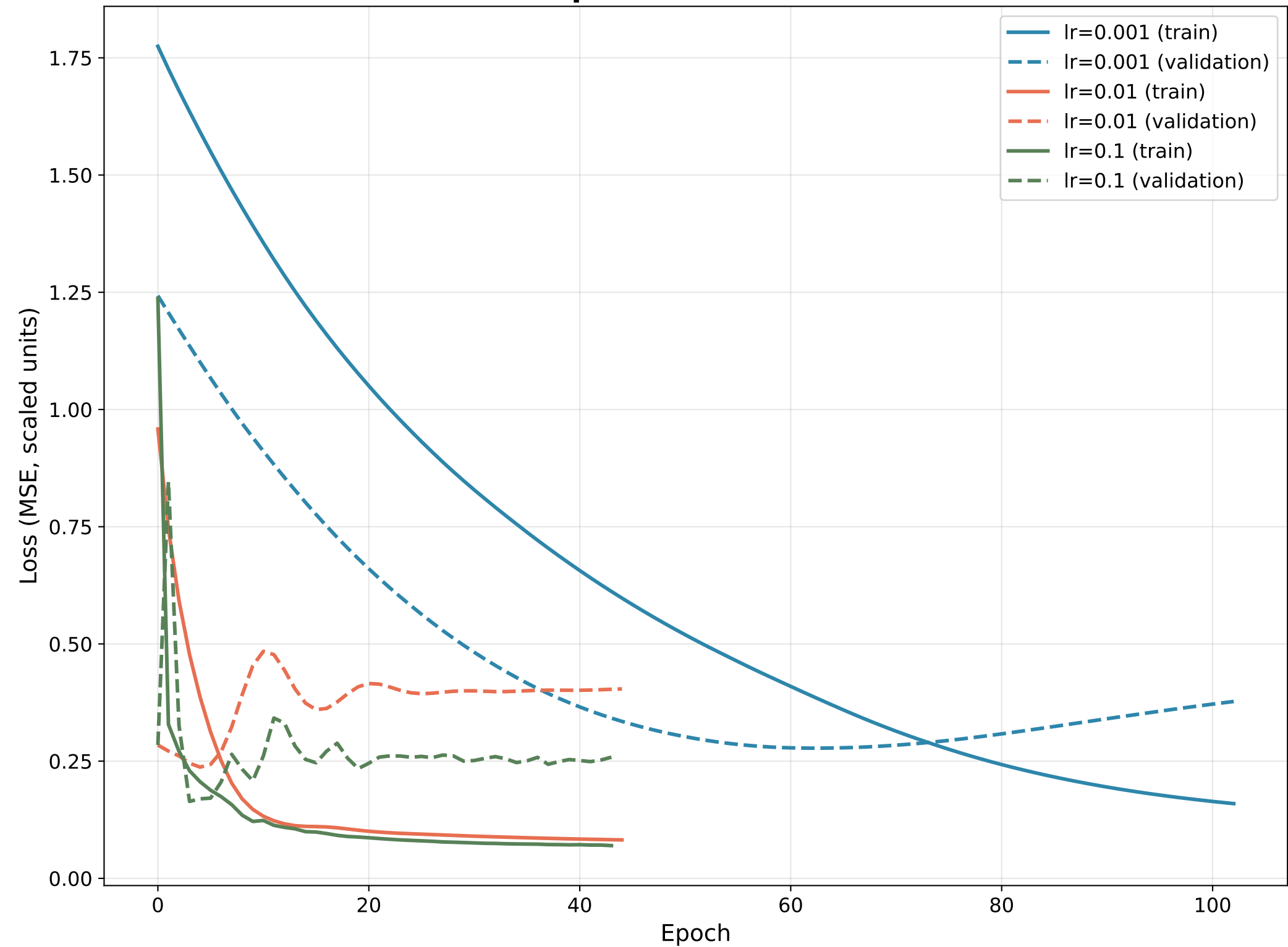
MSE vs. Epoch — activation = relu
