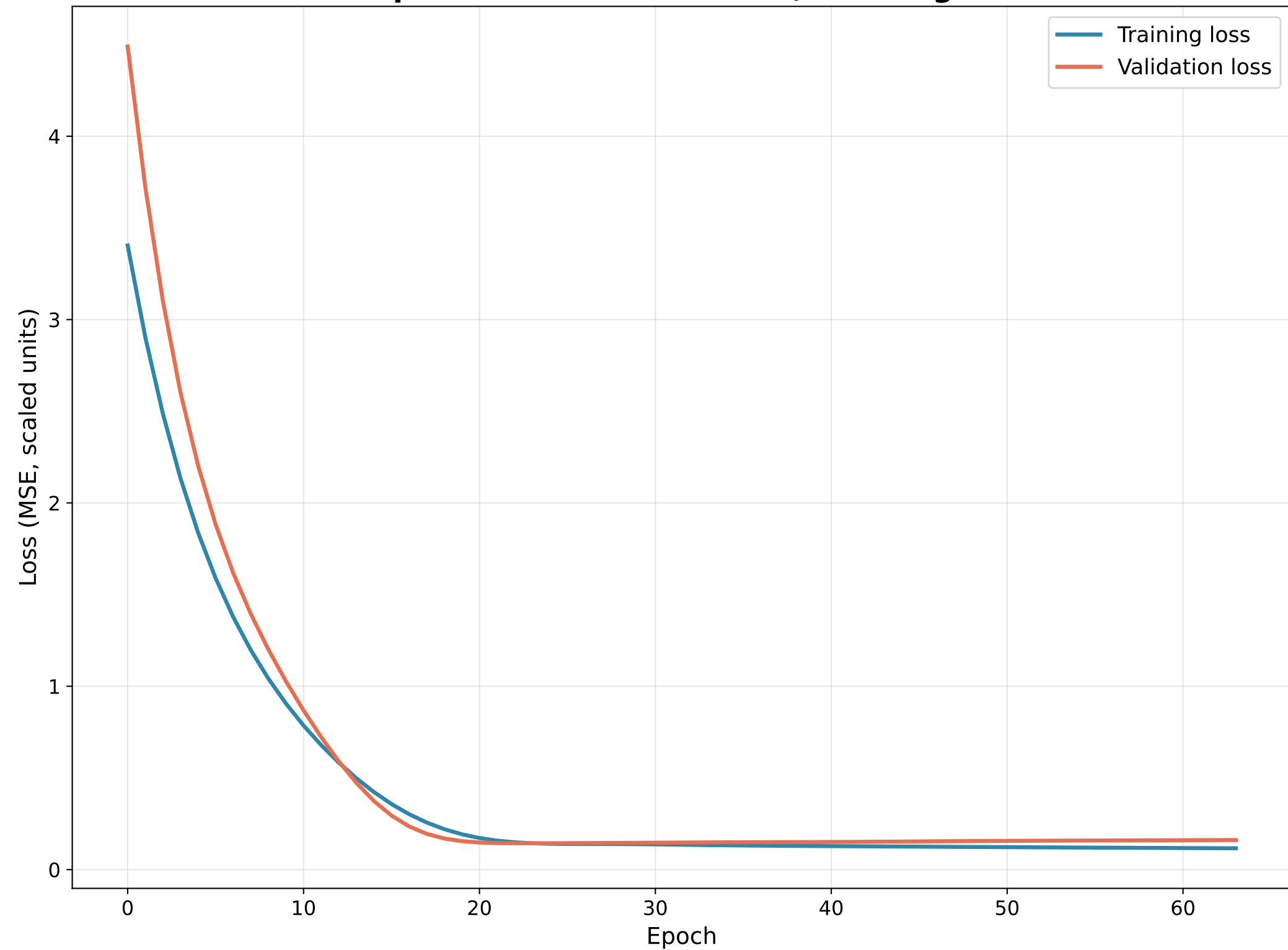
MSE vs. Epoch — activation=tanh, learning rate=0.01
