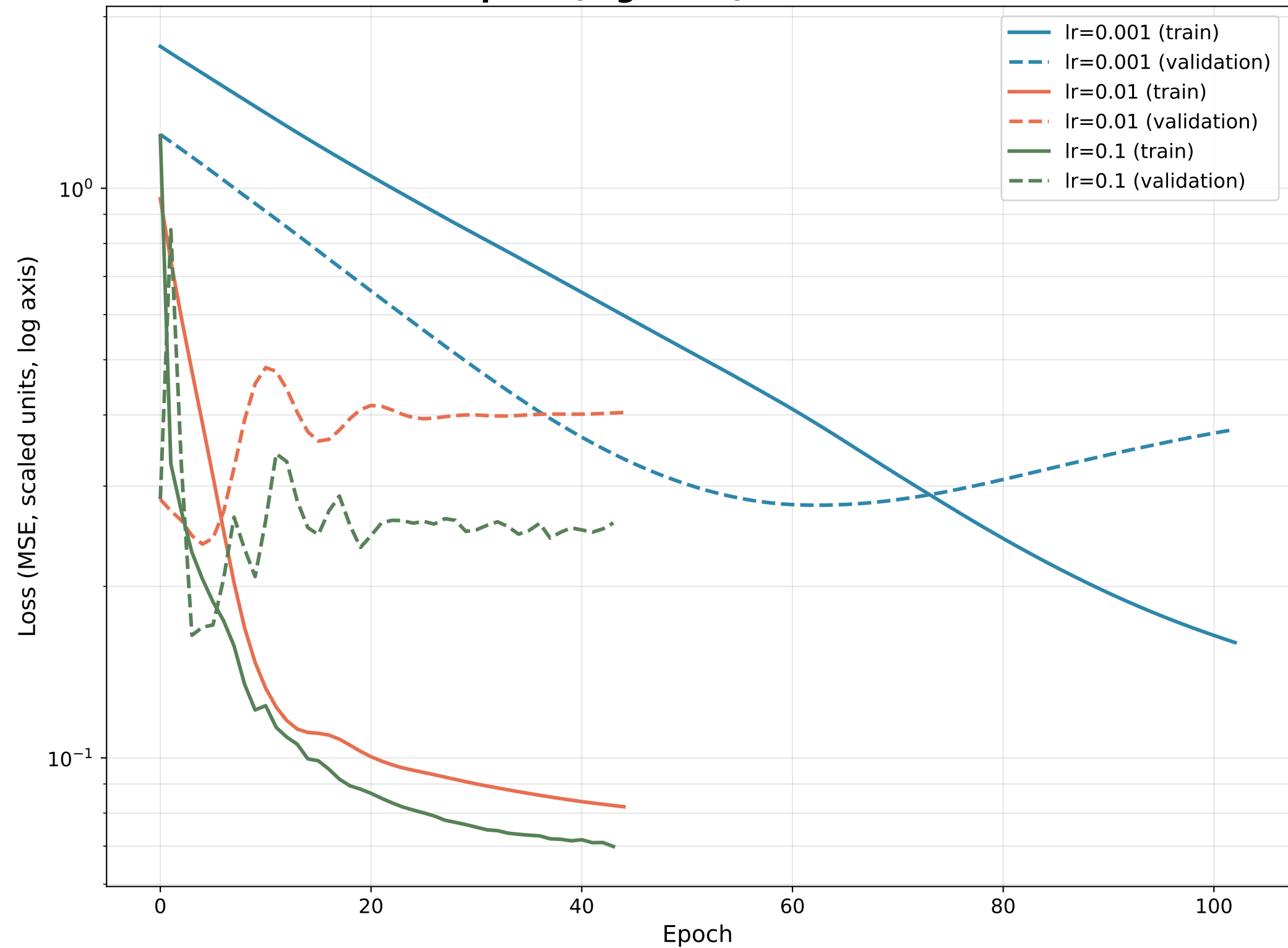
MSE vs. Epoch (log scale) — activation = relu
