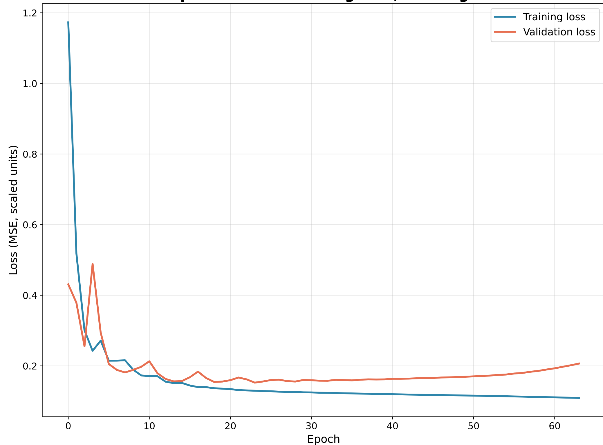
MSE vs. Epoch — activation=sigmoid, learning rate=0.1
