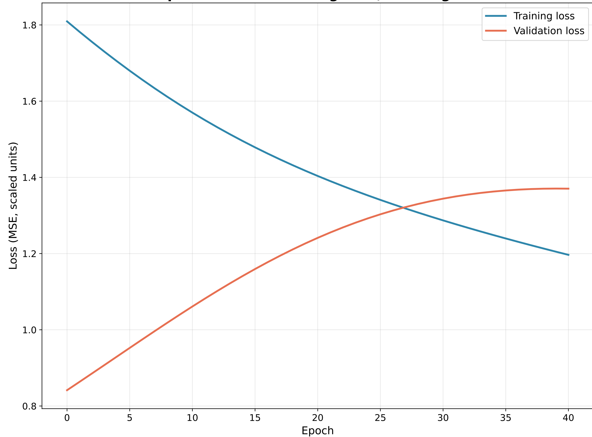
MSE vs. Epoch — activation=sigmoid, learning rate=0.001
