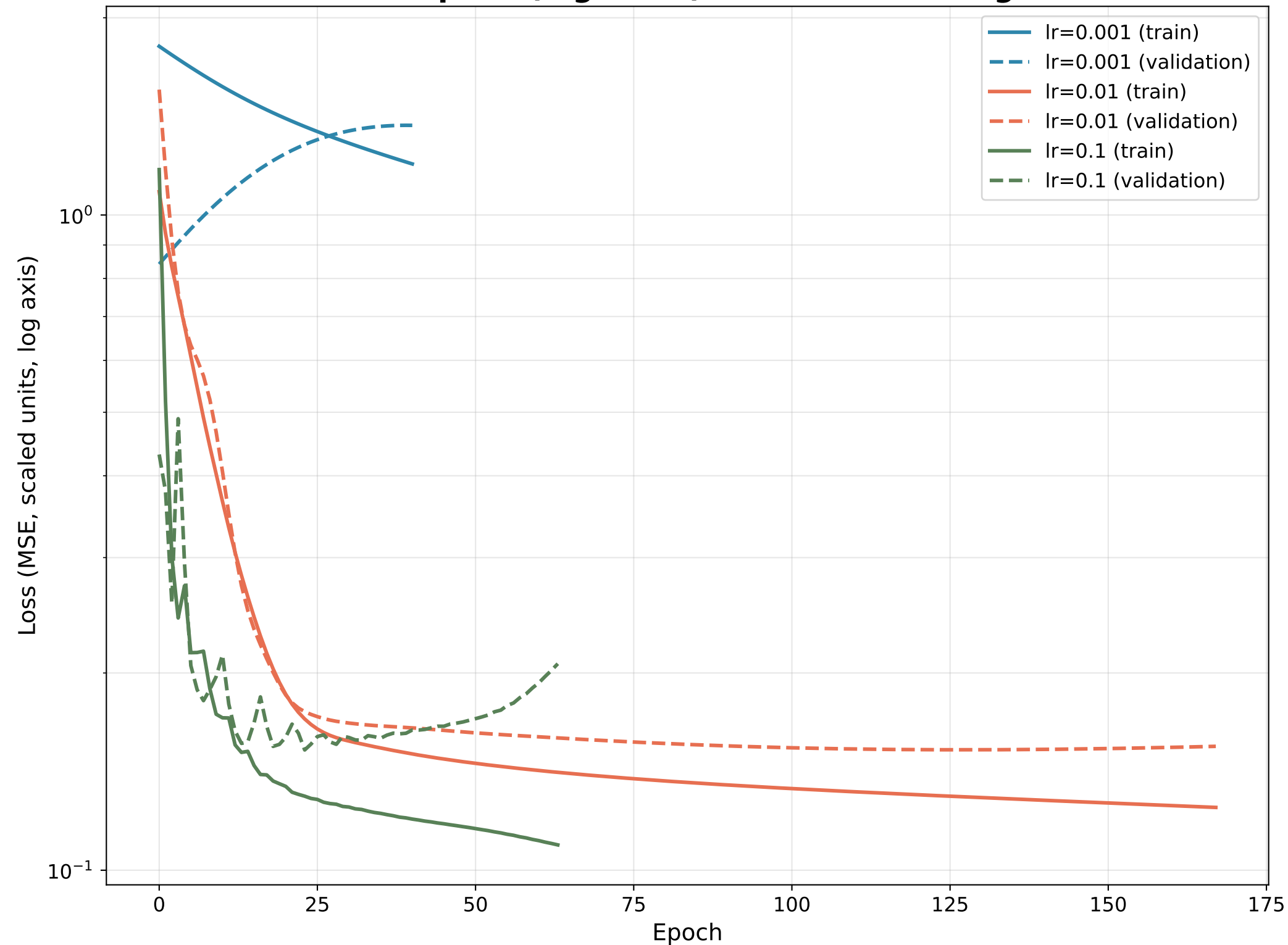
MSE vs. Epoch (log scale) — activation = sigmoid
