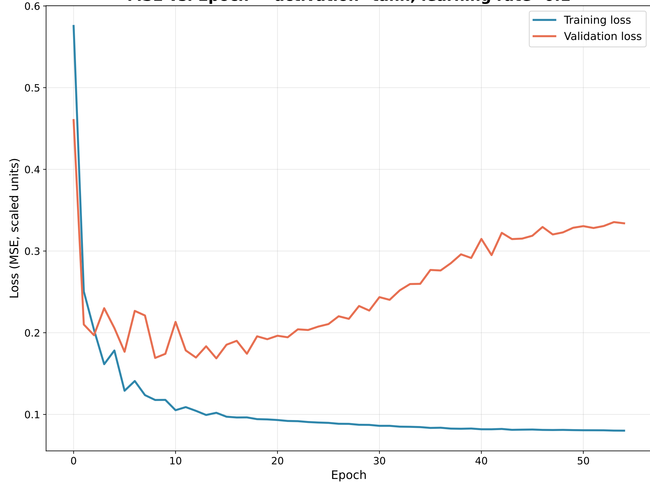
MSE vs. Epoch — activation=tanh, learning rate=0.1
