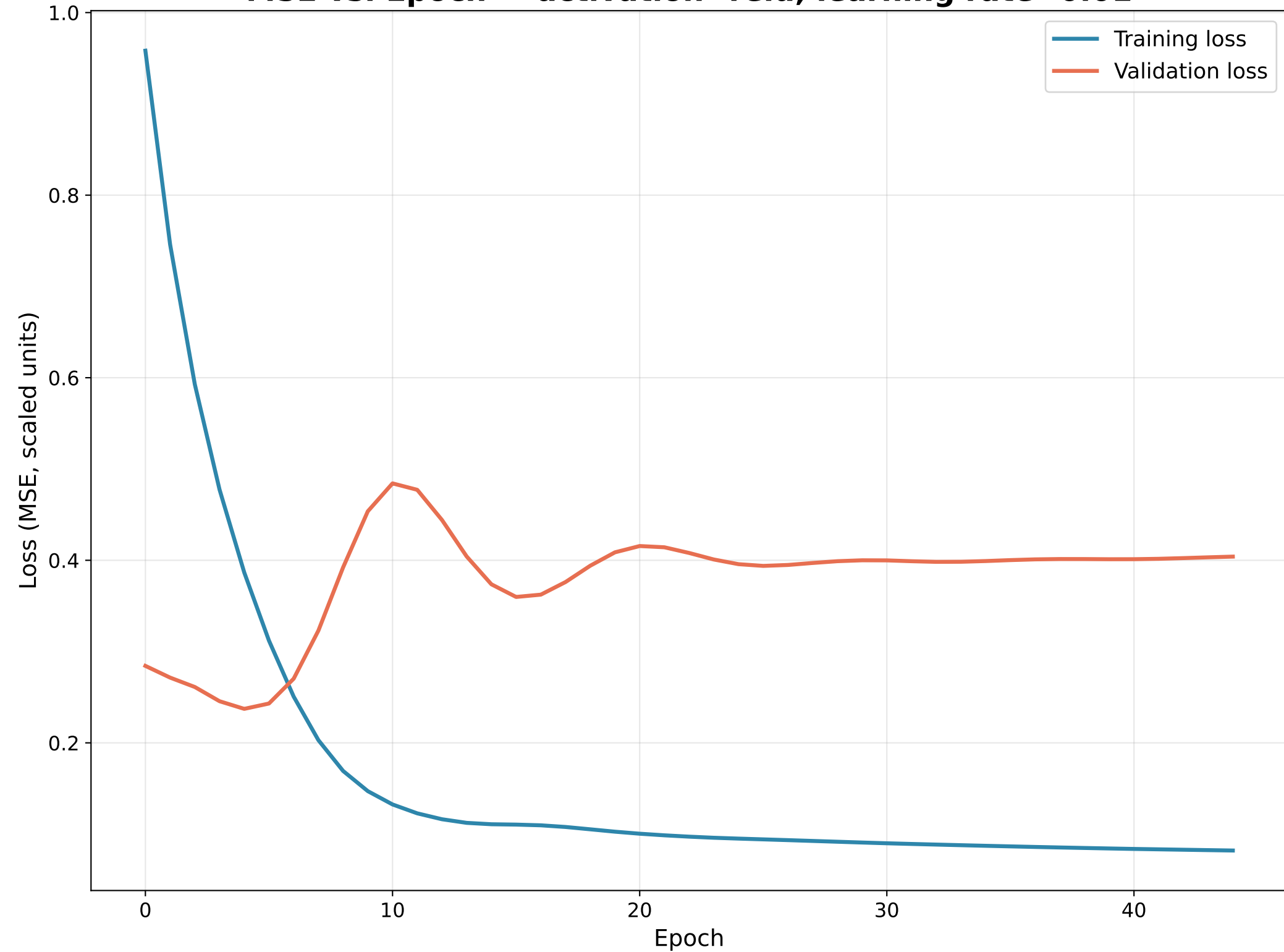
MSE vs. Epoch — activation=relu, learning rate=0.01
