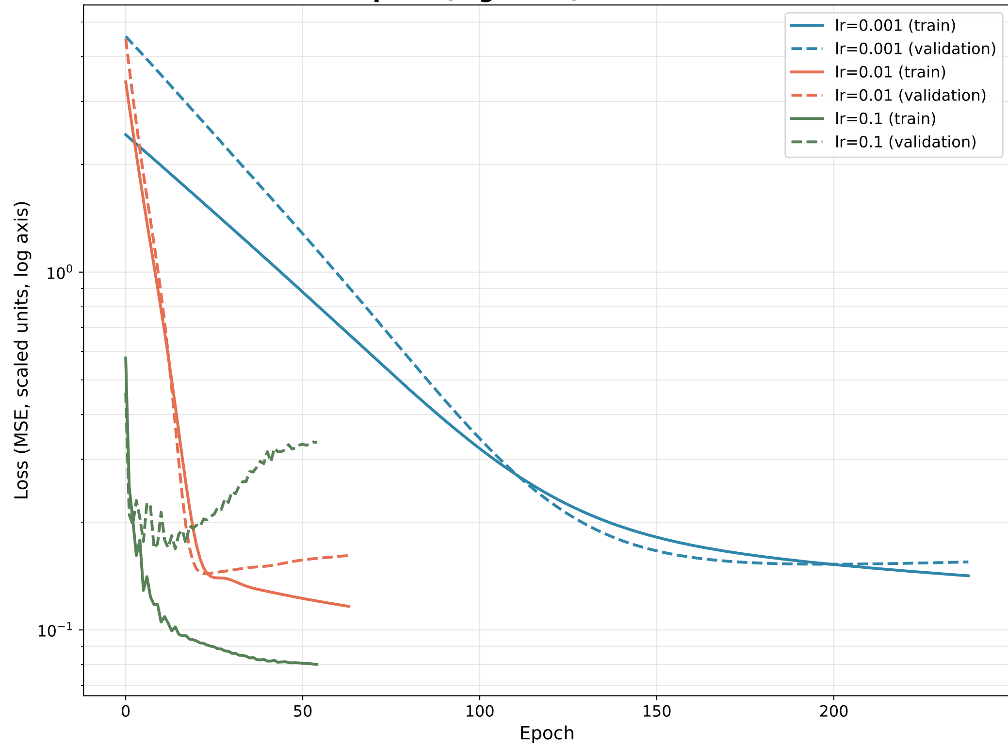
MSE vs. Epoch (log scale) — activation = tanh
