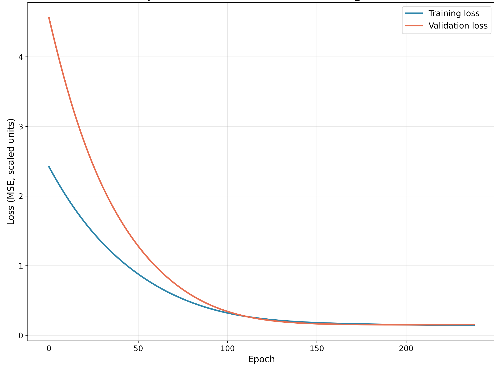
MSE vs. Epoch — activation=tanh, learning rate=0.001
