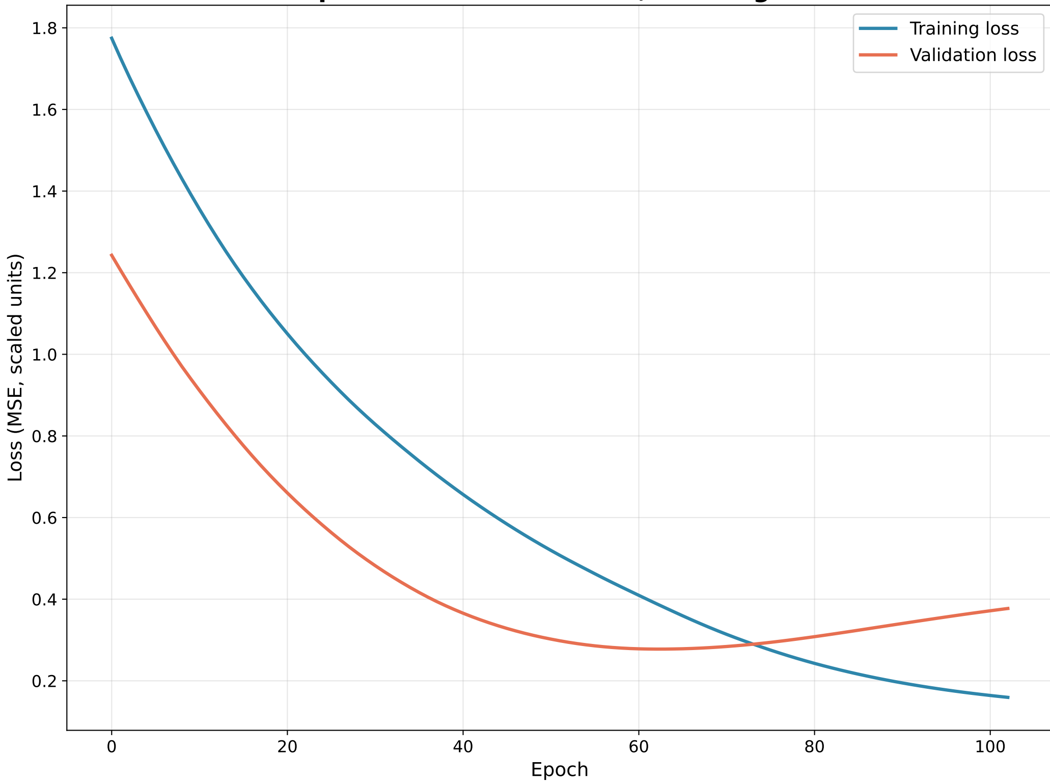
MSE vs. Epoch — activation=relu, learning rate=0.001
