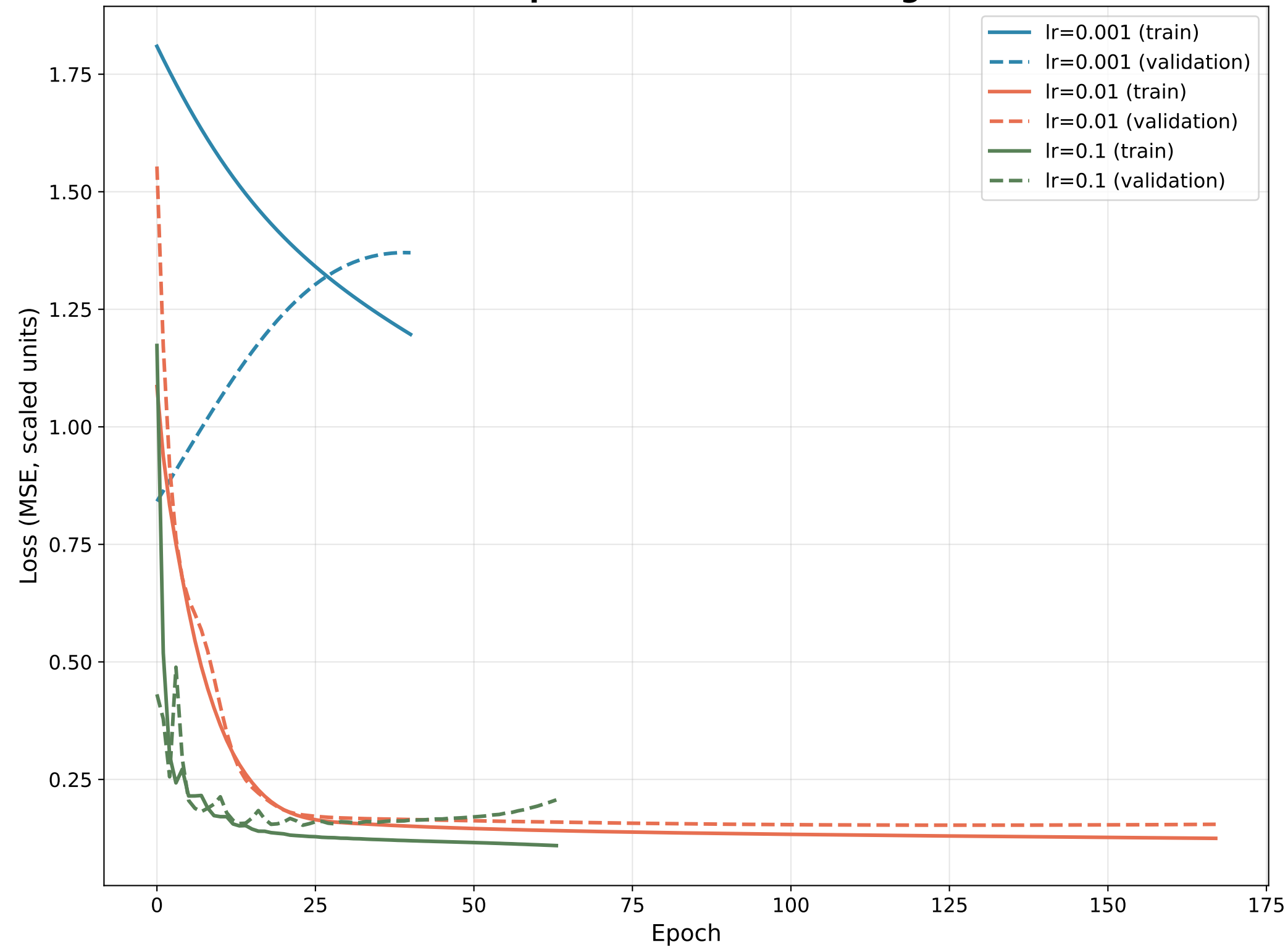
MSE vs. Epoch — activation = sigmoid
