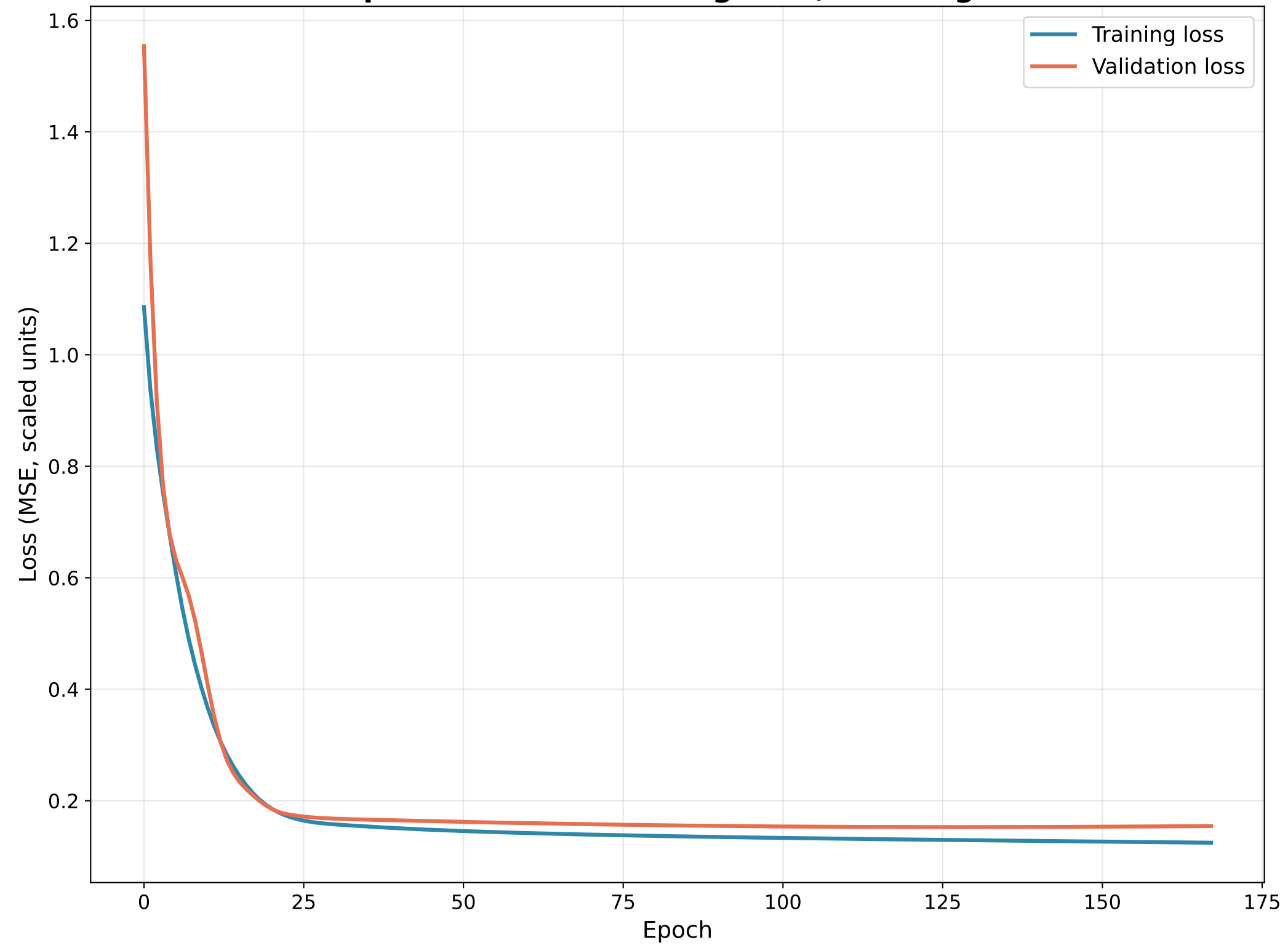
MSE vs. Epoch — activation=sigmoid, learning rate=0.01
