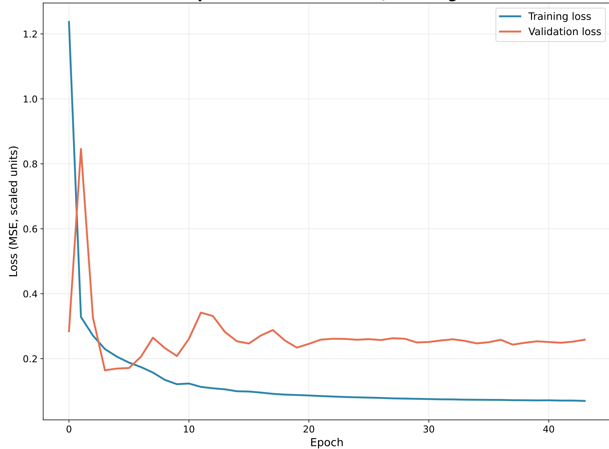
MSE vs. Epoch — activation=relu, learning rate=0.1
