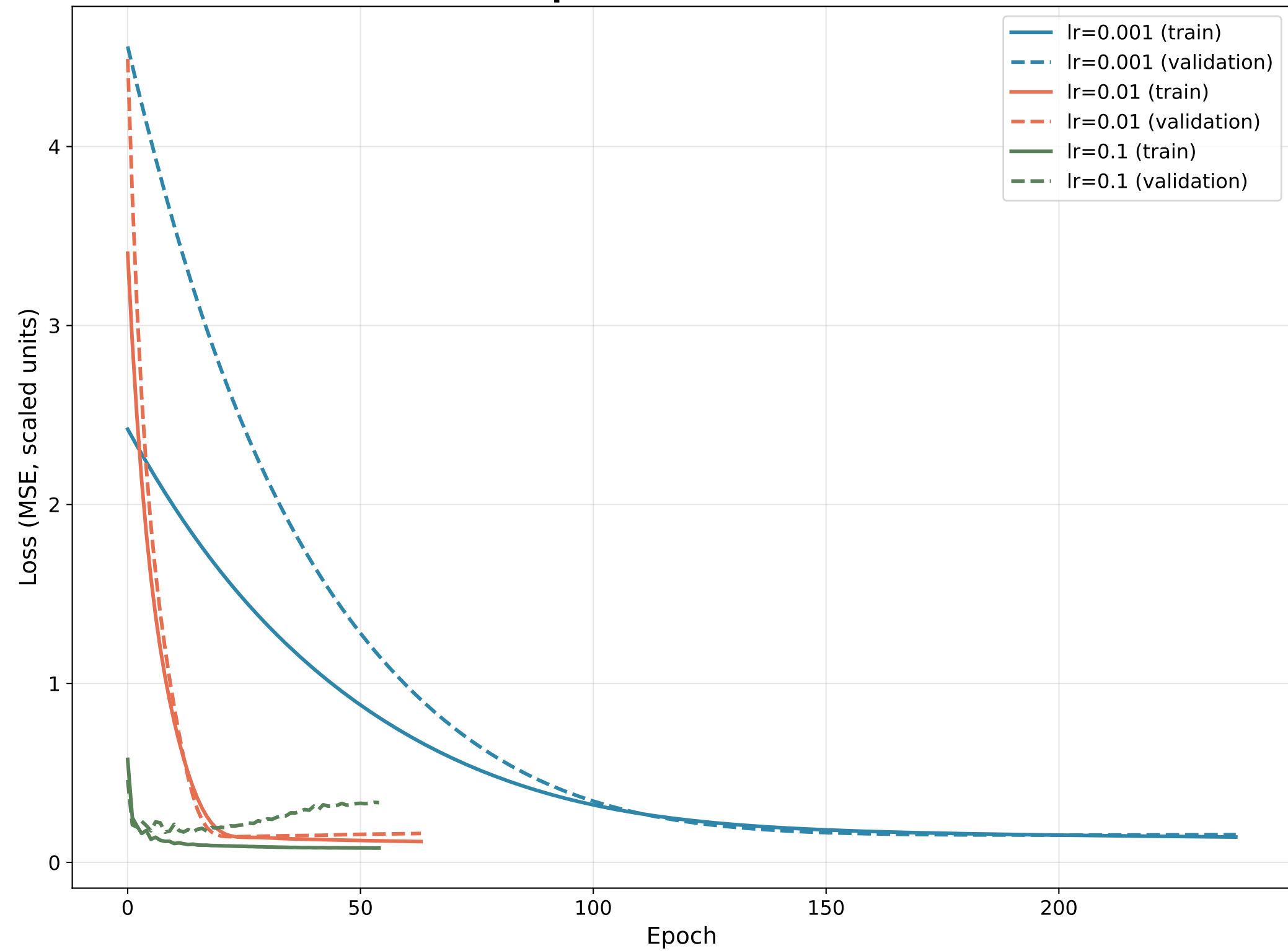
MSE vs. Epoch — activation = tanh
