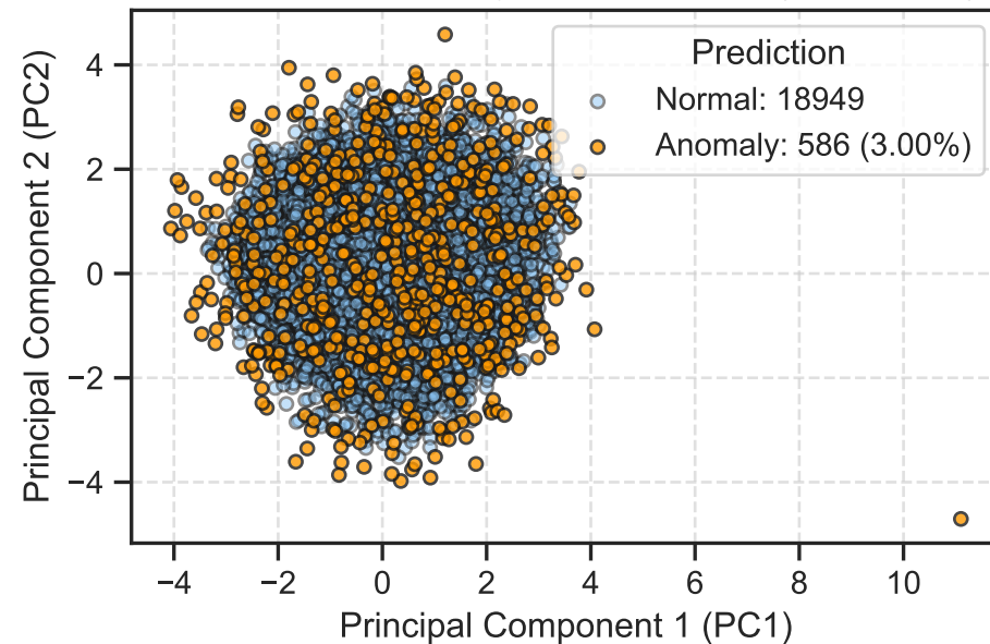
Anomalies Detected by OC-SVM Model (PCA Space)
