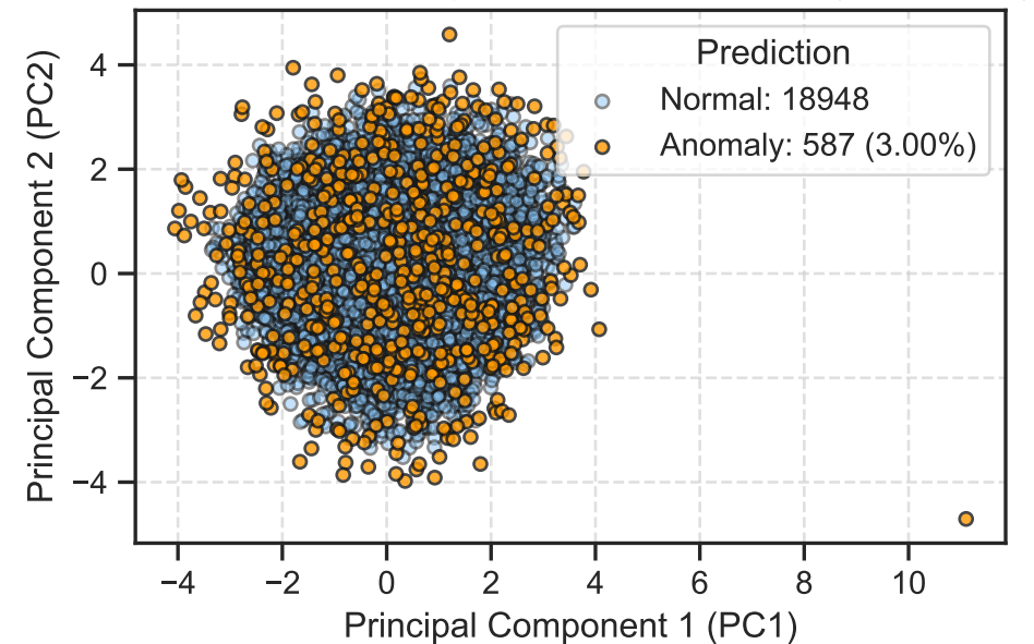
Anomalies Detected by Isolation Forest Model (PCA Space)
