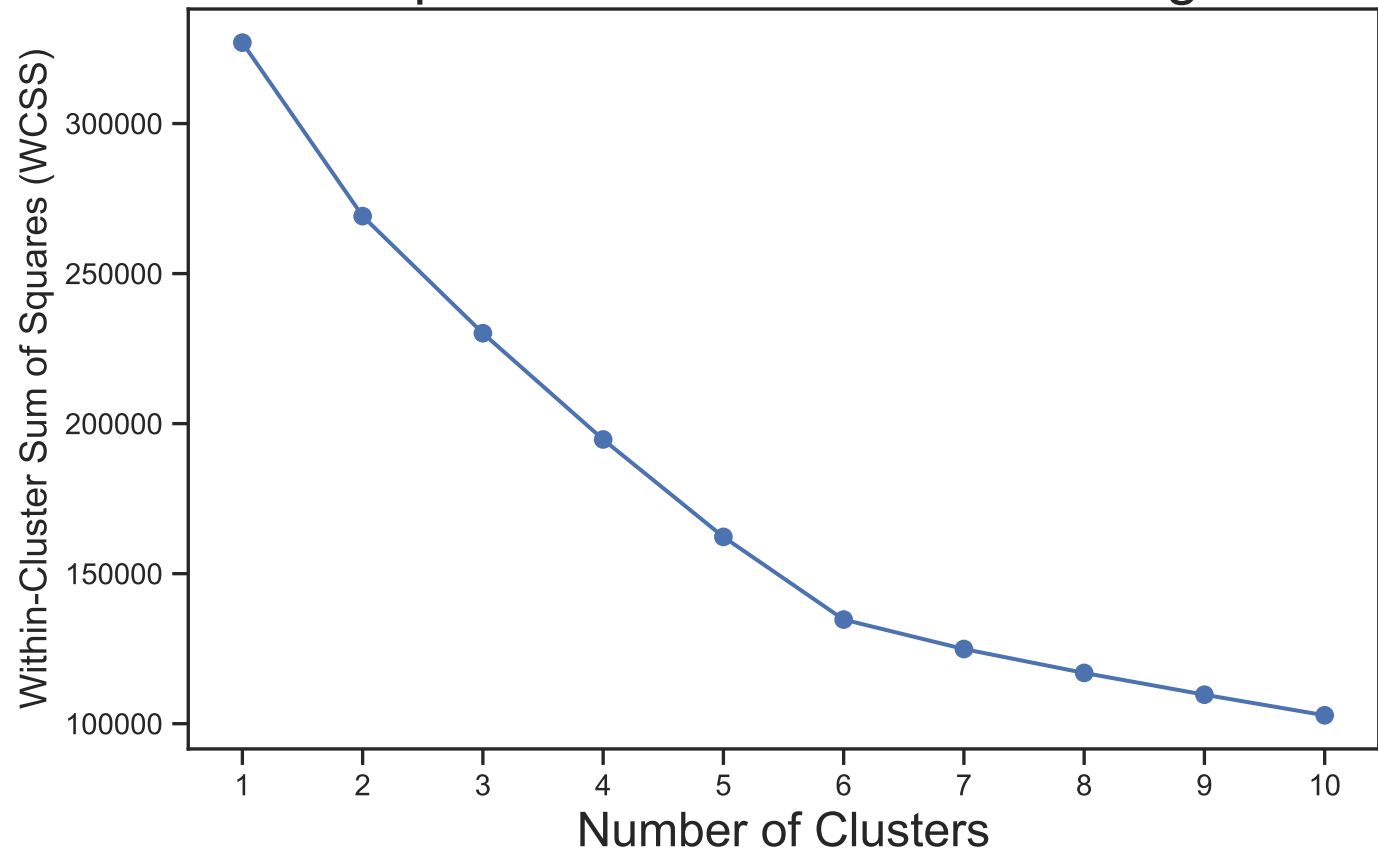
Optimal k with Standard Scaling
