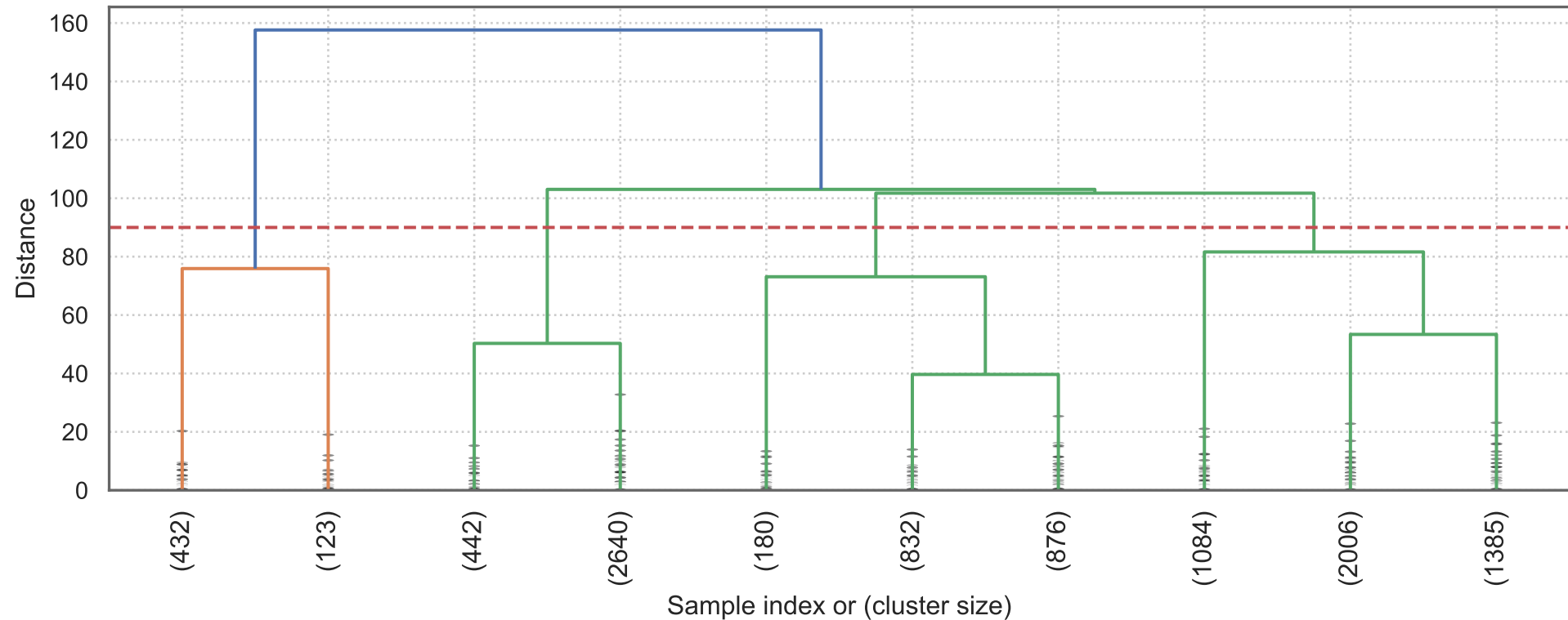
Hierarchical Clustering Dendrogram (Truncated)
