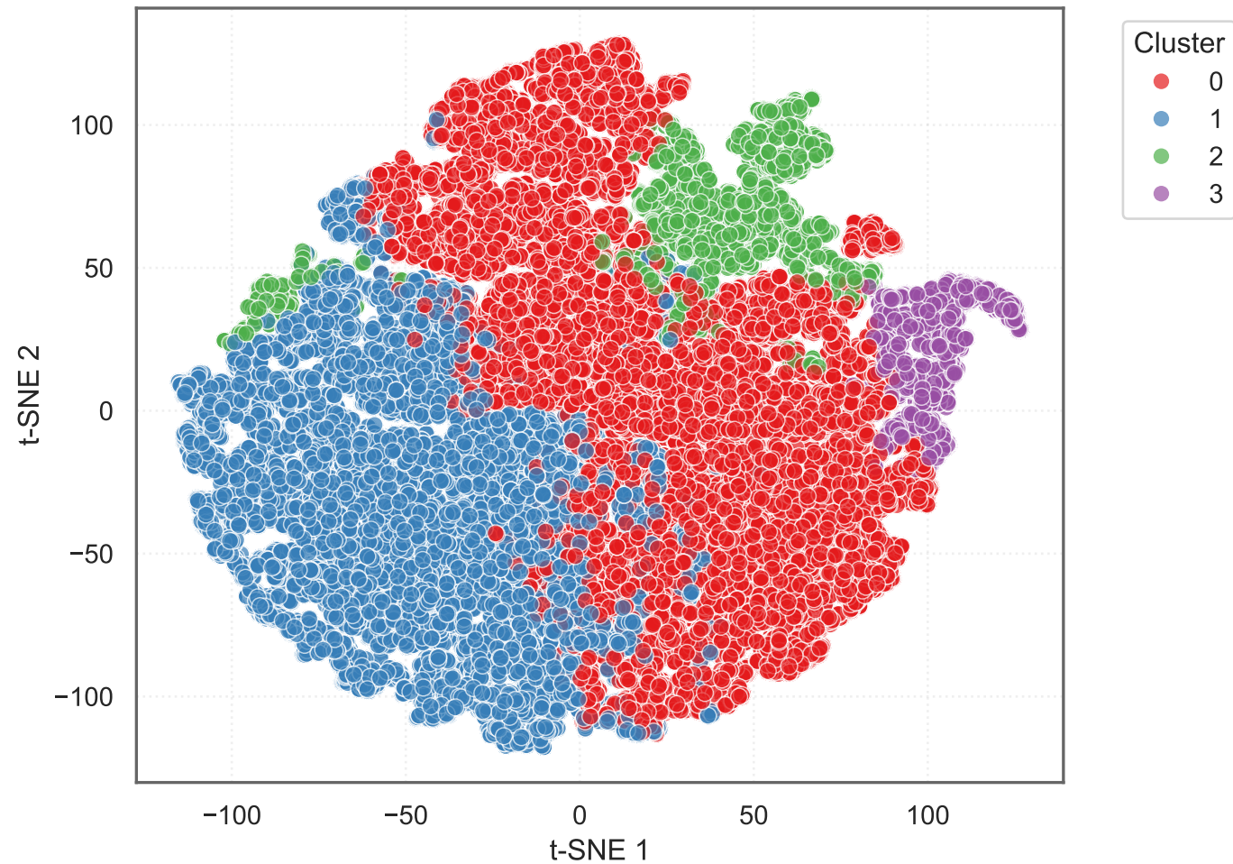
t-SNE with K-means Clusters (RobustScaler)
