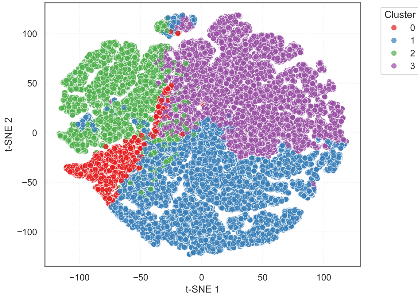
t-SNE with K-means Clusters (StandardScaler)
