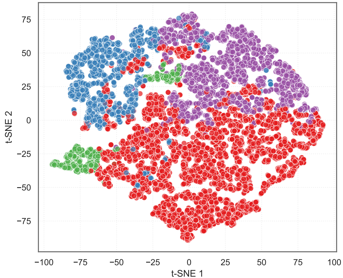
t-SNE with Hierarchical Clusters (StandardScaler)
