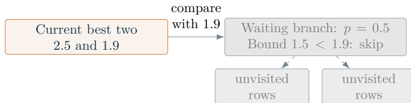
Figure 4: The whole gray subtree can be skipped because even its best possible score value is too low.
