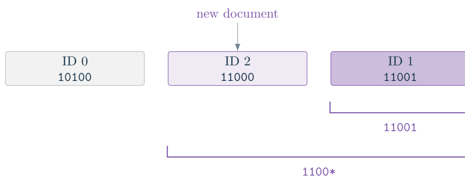
Figure 13: The broader prefix contains the previous range. ID 1 is already scored, so only the newly included document, ID 2, needs a scoring operation.
