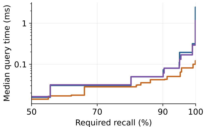
Return 1 document
