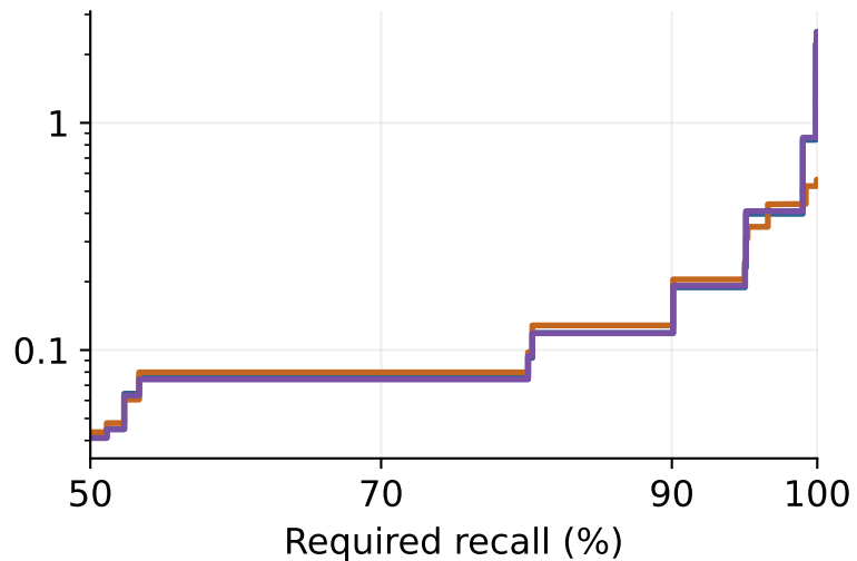
Return 100 documents
