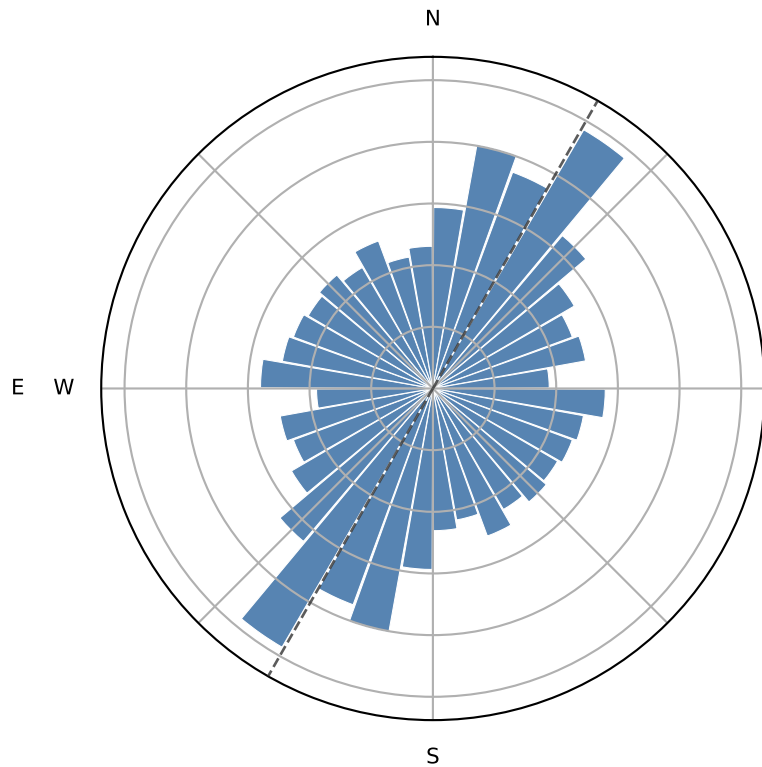
(b) RRB — cubeta alignment ( \theta_N ) n = 1431 · mean 30° · R = 0.13
