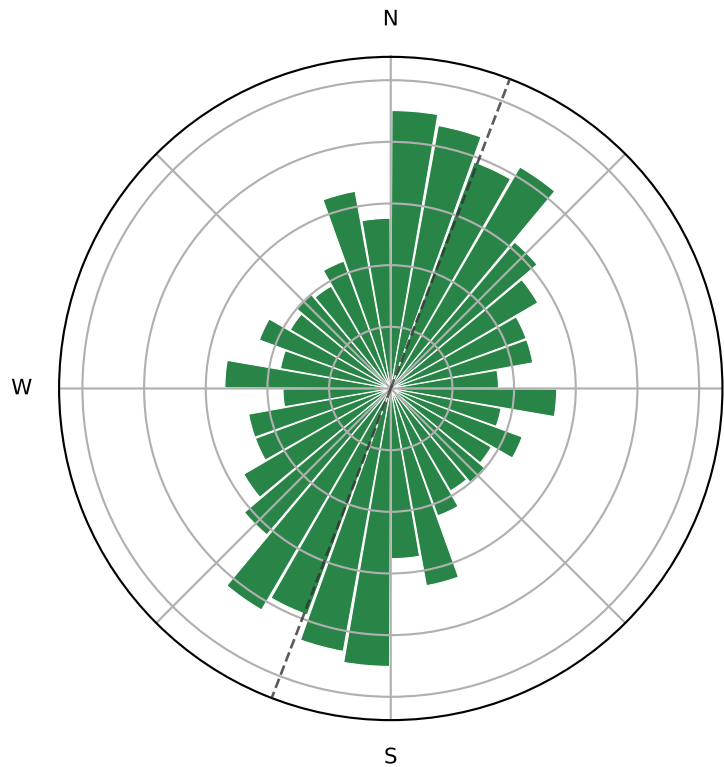
(a) RRB — cubeta orientation ( \theta_C ) n = 1431 · mean 21° · R = 0.19
