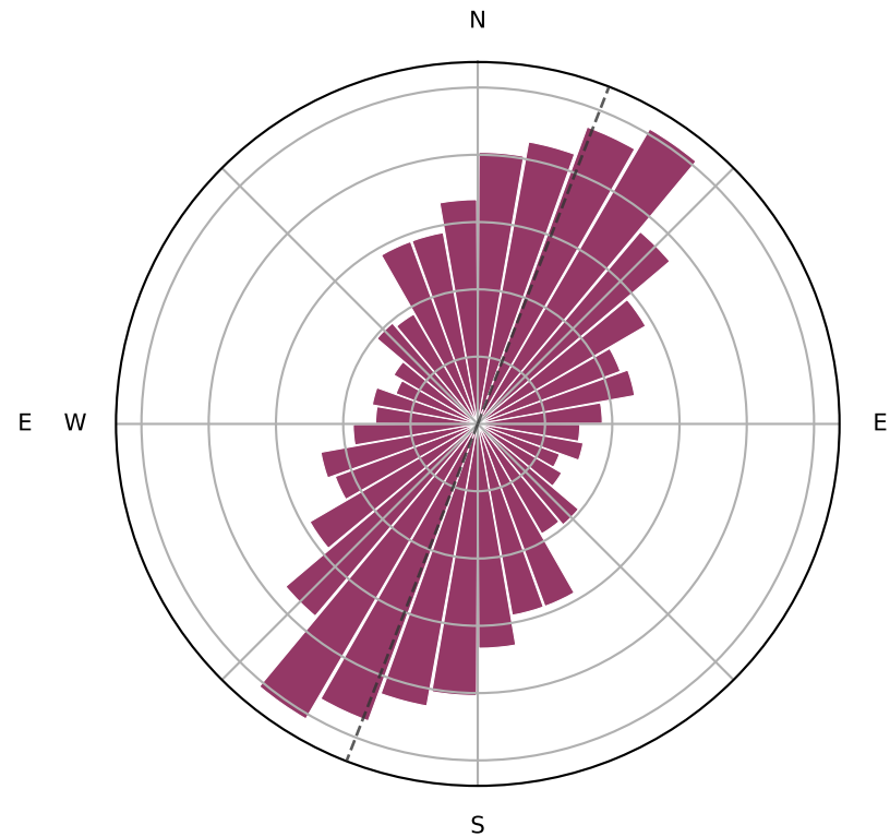
(c) RRB — valley orientation field ( \theta_V ) n = 1350 · mean 21° · R = 0.28
