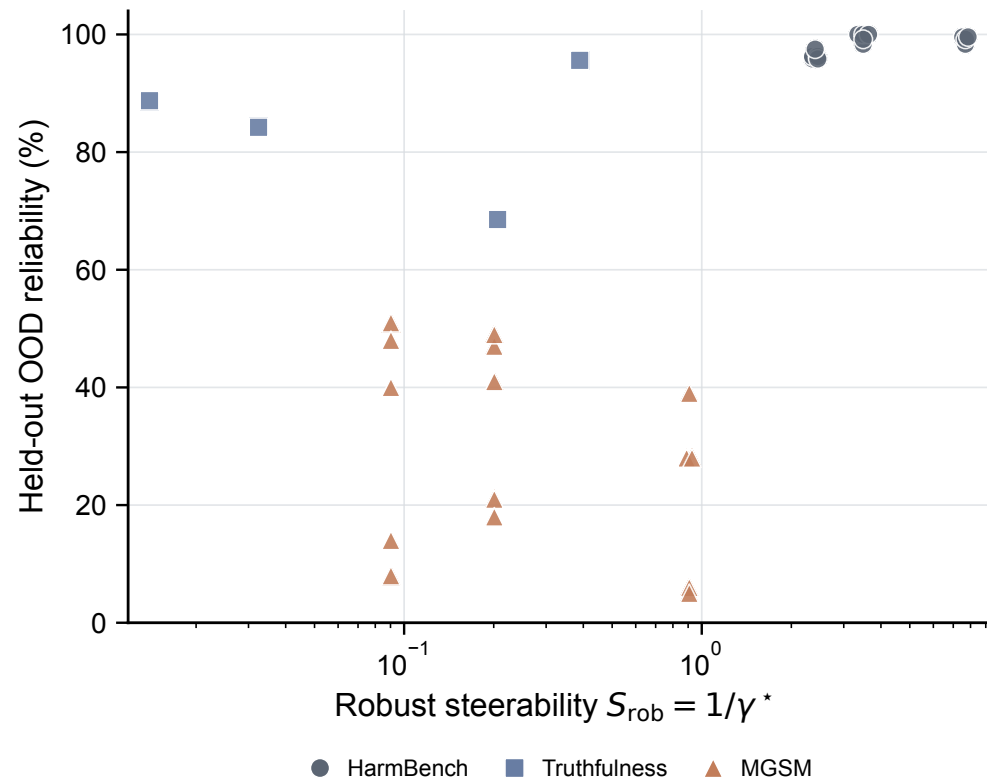
S_{\text{rob}} and OOD reliability
