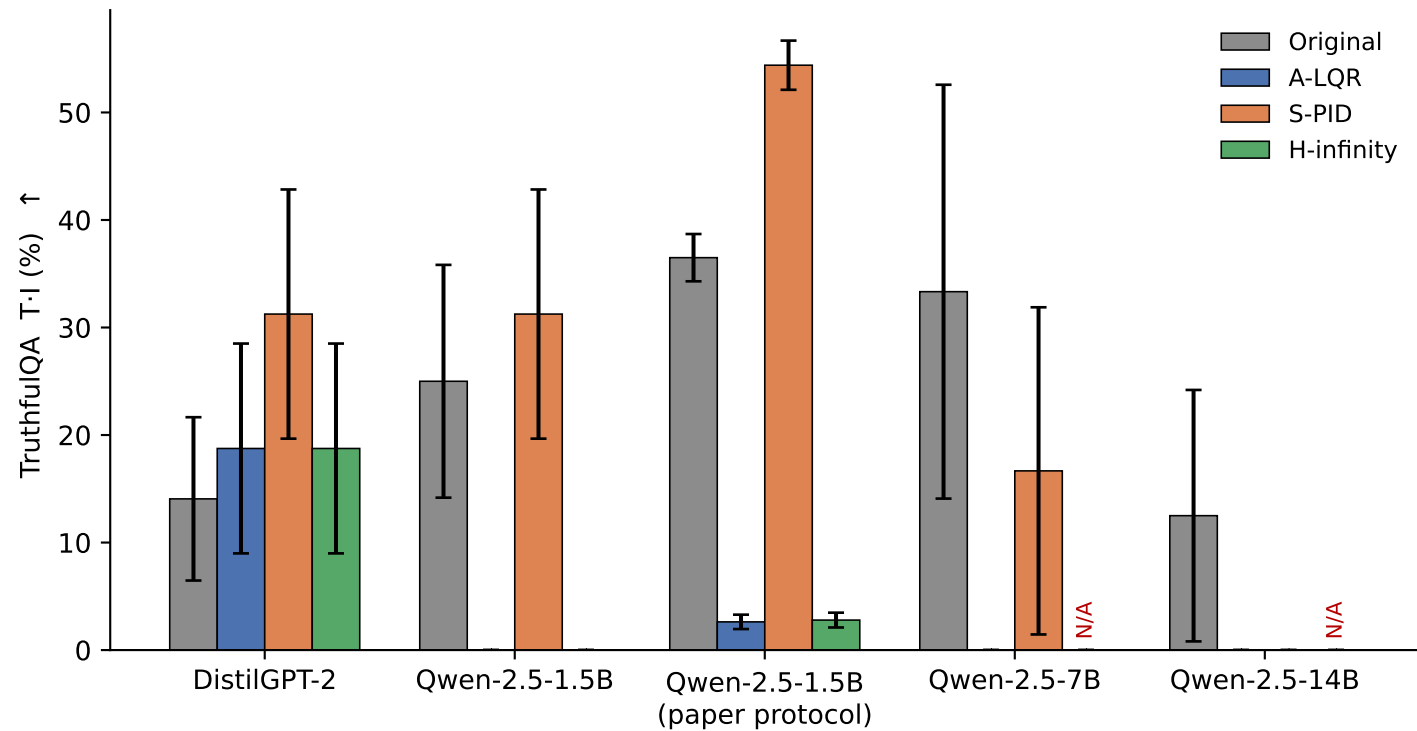
A. Truthfulness across model scales
