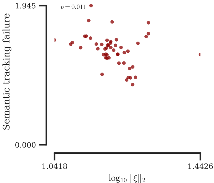
OOD: residual size, \rho = -0.36
